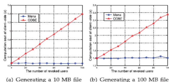
Fig. 2. Comparison on client computation cost for file generation between this scheme and ODBE.
