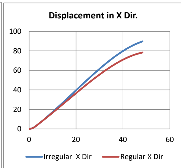
Graph No.2 Maximum displacement in x direction
