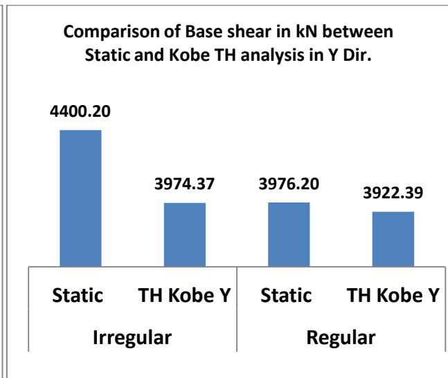
Graph No. 14 Base shear in kN in Y direction
