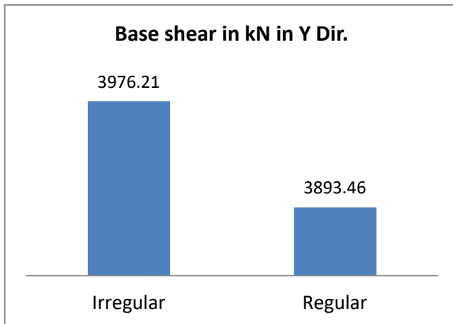
Graph No. 9 Base shear in kN in Y direction
