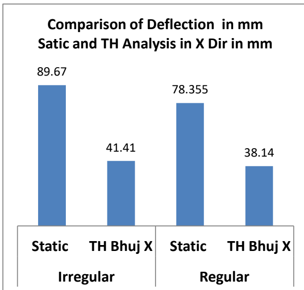
Graph No. 15 Maximum deflection in mm X direction
