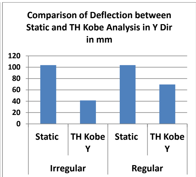
Graph No. 18 Maximum deflection in mm Y direction
