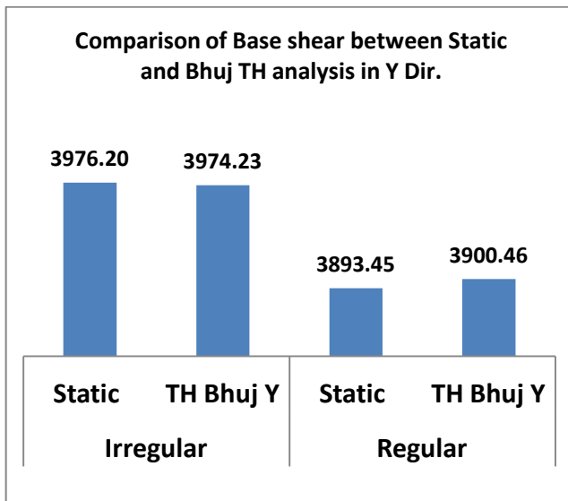
Graph No. 11 Base shear in kN in Y direction
