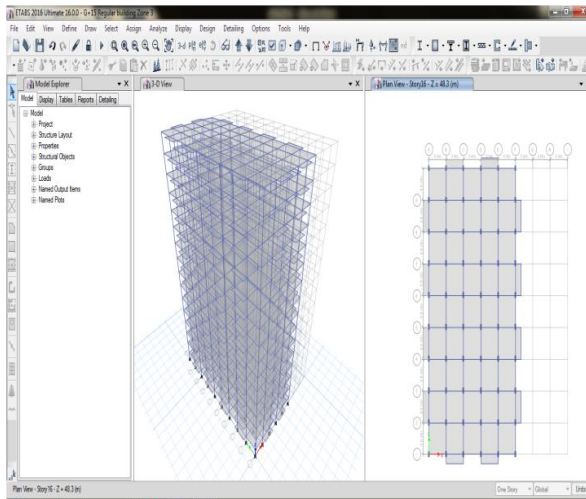
Figure No. 3.1 Regular Building
