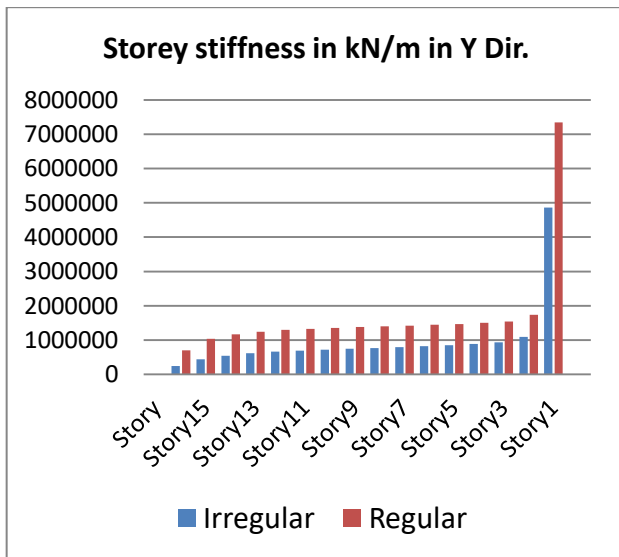
Graph No.7 Storesstiffness in Kn/m in Y direction
