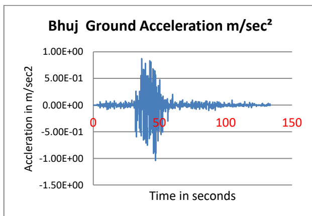
Figure No. 1 Bhuj ground acceleration
