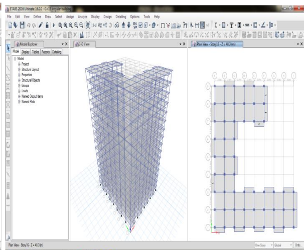
Figure No. 3.2 Irregular Building Modeling of Building
