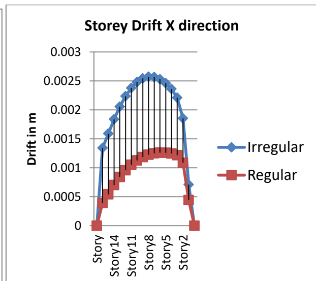
Graph No.4 Storey drift in m in X direction
