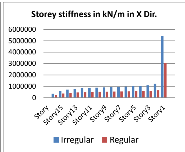
Graph No. 6Storesstiffness in Kn/m in X direction
