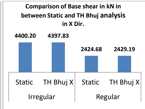
Graph No.10 Base shear in kN in X direction
