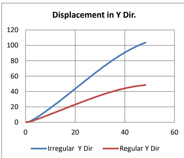
Graph No.3 Maximum displacement in Y direction
