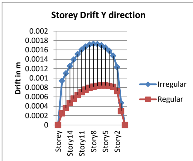
Graph No.5Stores drift in m in Y direction
