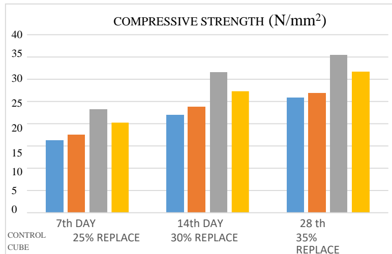
Figure 1. Compressive strength of replaced waste ceramic tiles
