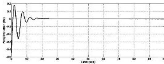
Fig. 11. Simulation result with PID controller
