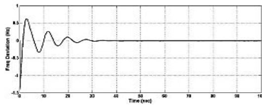
Fig. 10. Simulation result with PI controller
