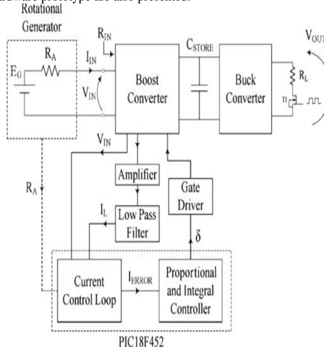
Figure: 2 Adaptive Maximum Power Point Tracking
