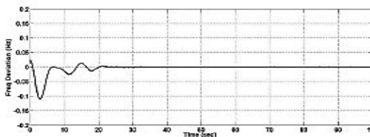
Fig. 12. Simulation result with Fuzzy controller
