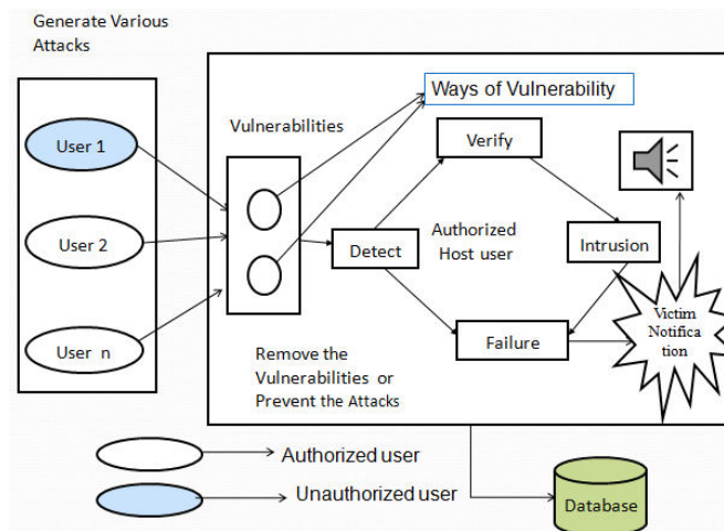
Fig 1. Architecture Diagram for ZDAP System
