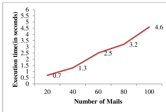
Fig 6. Execution Time of e- mail Abstraction Generation of the System
