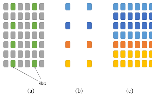
Fig. 1. (a) Resource grid with pilots (b) Extracted pilot symbols that were affected by the channel (c) Channel estimation based on the extracted pilots
