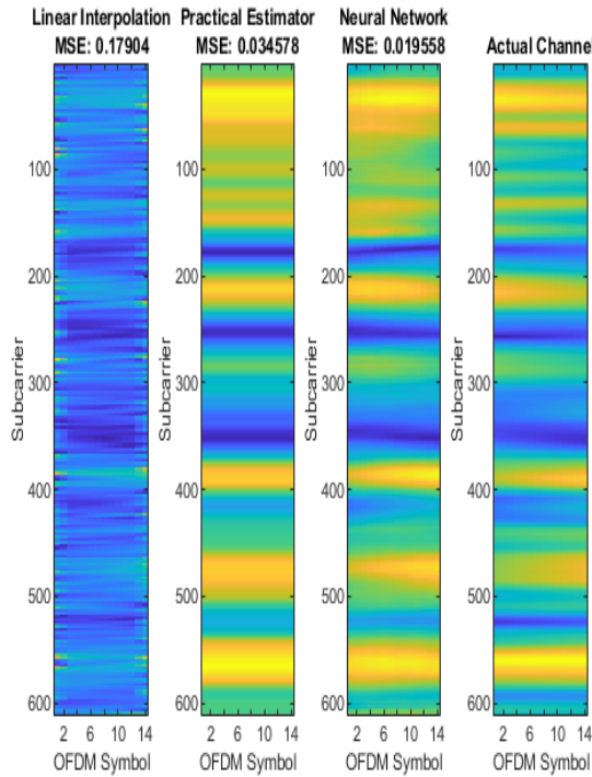
Fig. 3. Channel estimation Output with various models.
