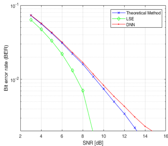
Fig. 4. Bit error rate vs SNR for channel estimation with the proposed method as well as some conventional methods.
