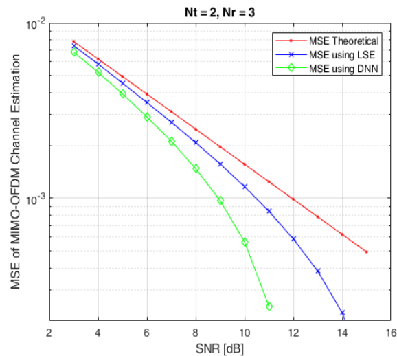
Fig. 5. Mean square error (MSE) while estimating channel vs SNR for proposed method as well as other channel estimation methods.
