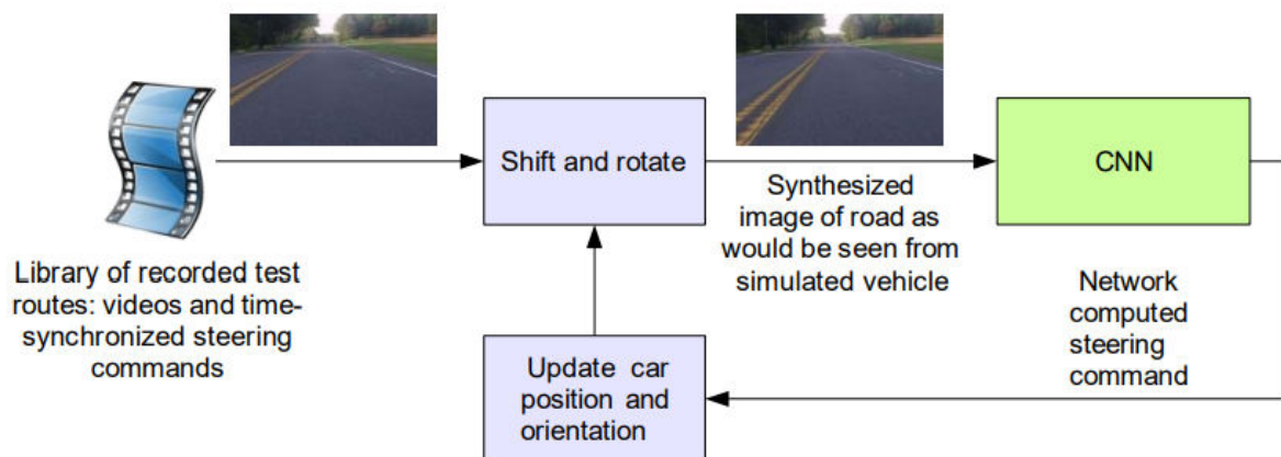
Figure 5: Block-diagram of the drive simulator.
