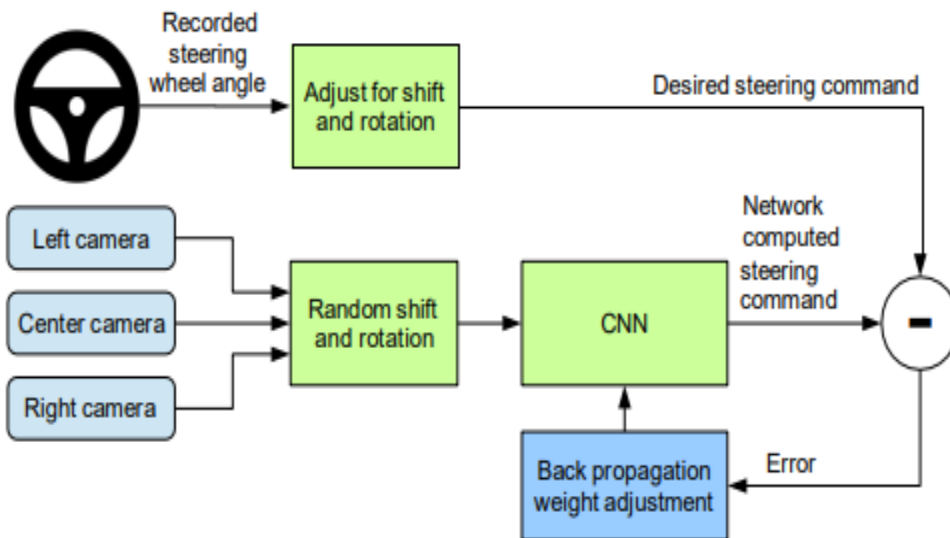
Figure 2: Training the neural network.
