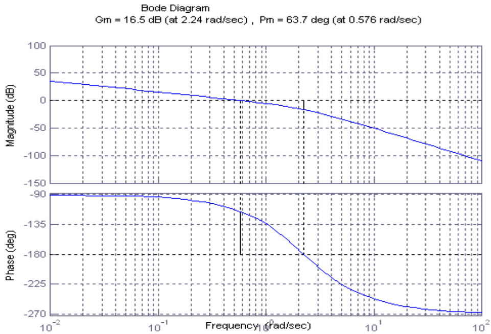
Fig.3 Bode plot of uncompensated system
