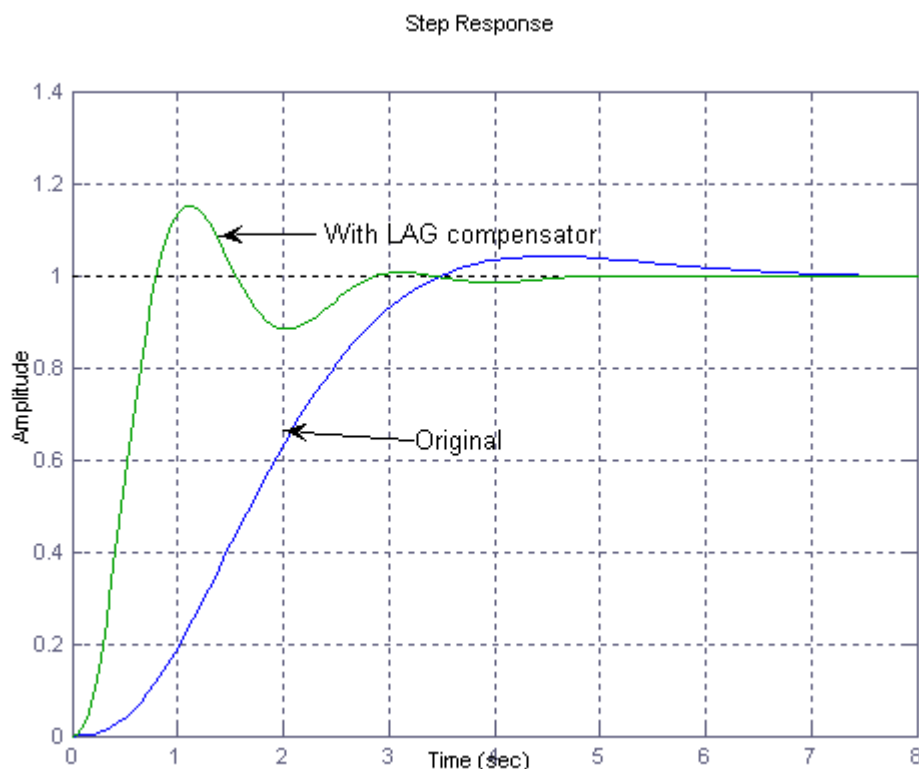
Fig.5 Step response of the system
