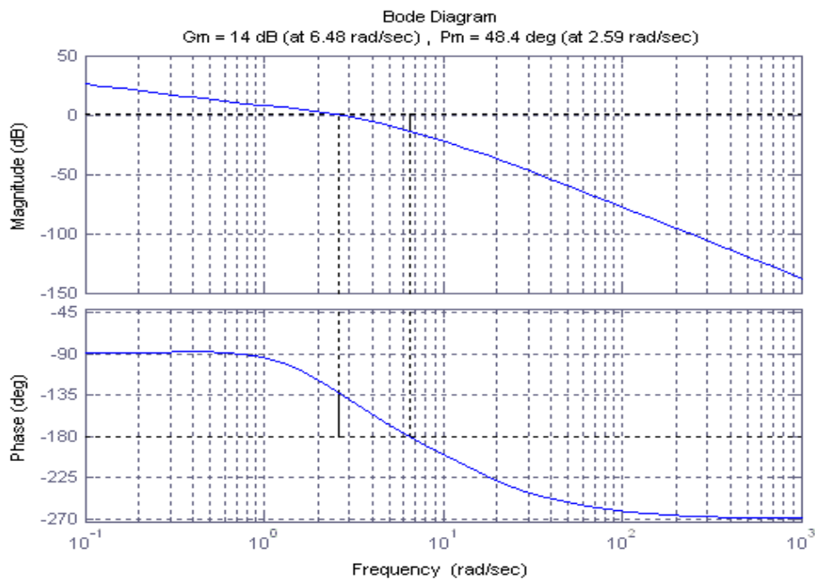
Fig.4 Bode plot of compensated system
