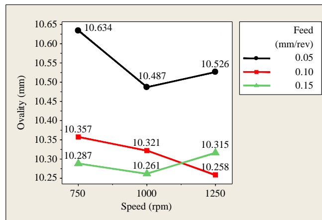
Fig. 8 Influence of feed and spindle speed on average ovality
