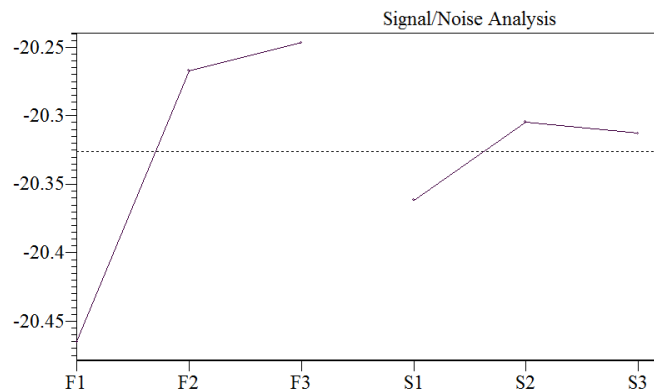
Fig. 9 Response graph of ovality for process parameters in drilling nonlaminated GFRP composite rods
