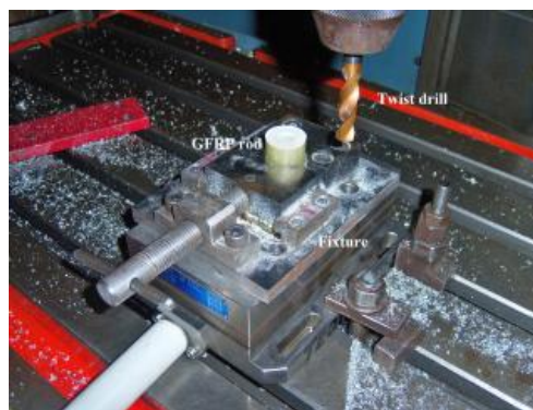
Fig. 5 Close-up photograph of the experimental setup
