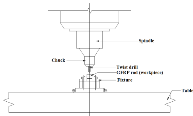
Fig. 6 Schematic representation of experimental setup
