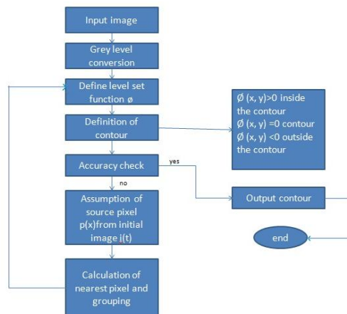
Fig 3. Flow chart for hybridization
