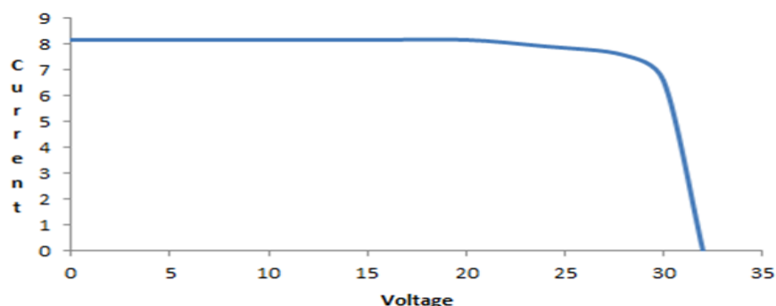
Fig 4 Solar photovoltaic characteristics
