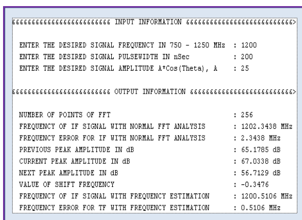
Fig. 4: MATLAB Frequency Estimation, 256 Points FFT
