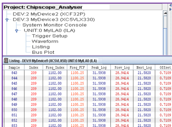
Fig. 6: ChipscopePro Result of Frequency Estimation Pulse width 200 nSec and -40 dBm
