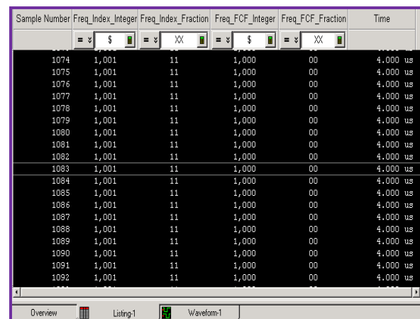
Fig. 7: LSA Result of Frequency Estimation Pulse width 200 nSec, and -40 dBm
