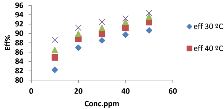
Fig.7: The relation between inhibition efficiency of Metronidazole and its concentrations against the molar conductance of 0.5M HCl at different temperatures.
