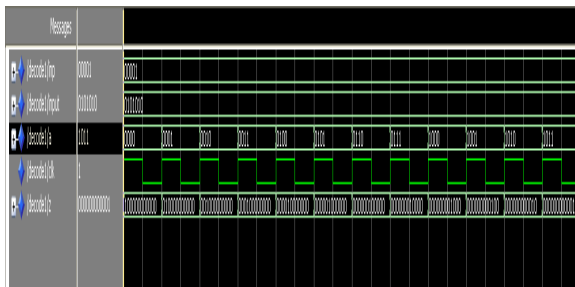
Figure 8: 4:12 Decoder
