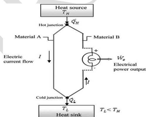
Figure 7- Circuitry of thermoelectric power
