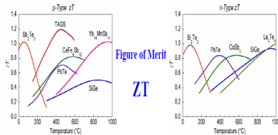
Figure 3- Figure of merit ZT
