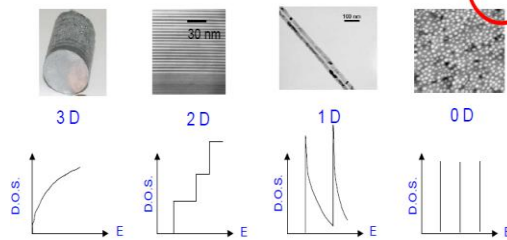
Figure 4- Dimensional view of material
