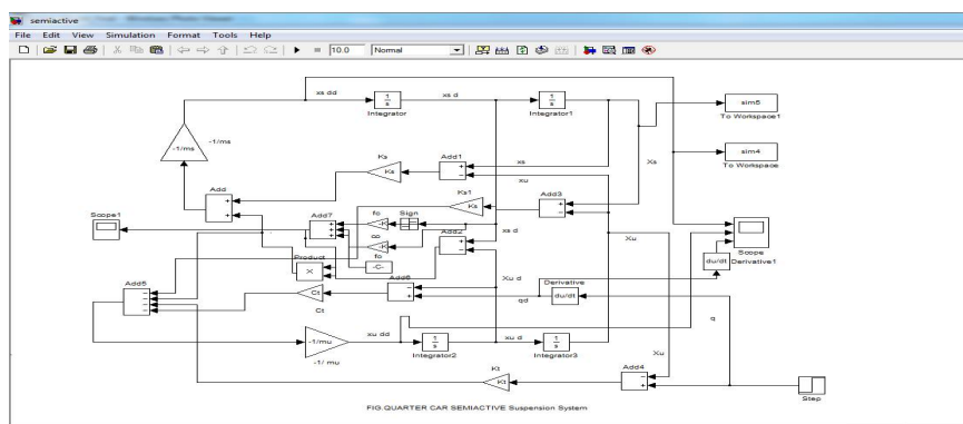
Figure5 : MATLAB/Simulink Model of Semiactive Suspension System based on Bingham Model
