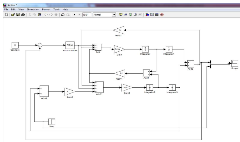
Figure 6 : MATLAB/Simulink Model of active Suspension System based on Bingham Model
