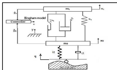
Figure 4: Quarter car vehicle with MR damper
