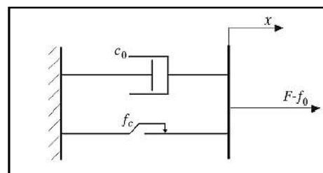
Figure 3: Schematic of Bingham model
