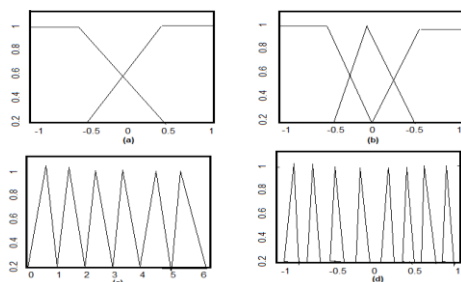
Fig 4. Fuzzy membership functions. (a) flux error, (b) torque error, (c) stator flux position sector, (d) pulses controlling the pwm inverter.
