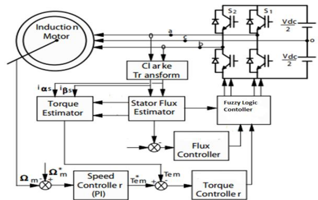
Fig 5. Block Diagram of fuzzy logic DTC.
