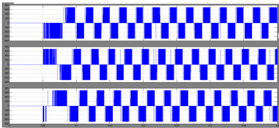
Fig.(a).Proposed stator voltage(Vas)
