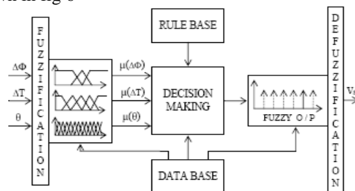
Fig.6:DTFC functional Block diagram
