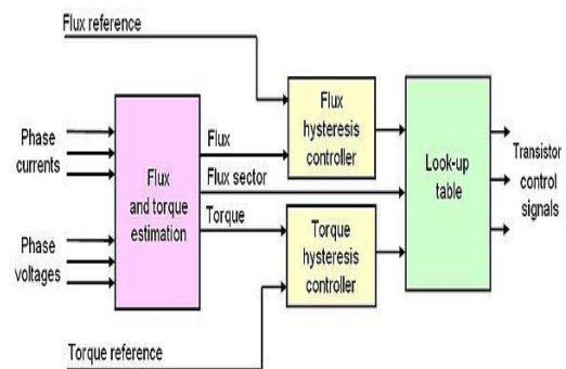
Fig.2. Control Method
