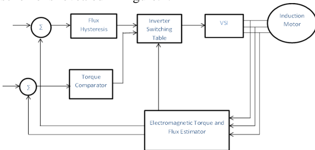
Fig.1. Block Diagram of DTC.
