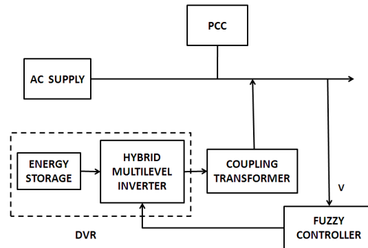
Figure.1 Block diagram
