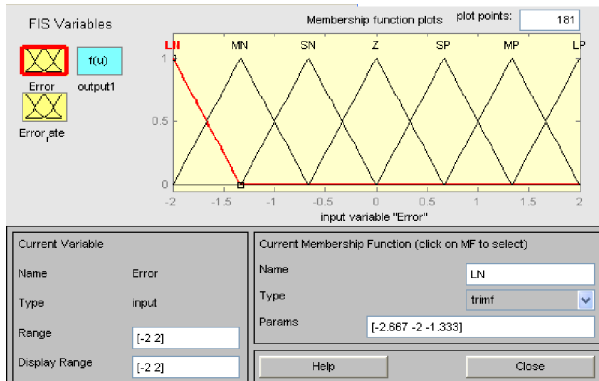
Figure. 3 Membership functions of fuzzy controller
