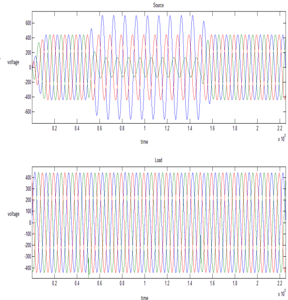
Figure. 7 Three phase source and load voltage
