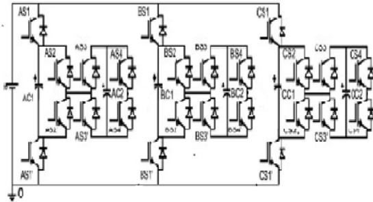
Figure.2 Hybrid multilevel inverter
