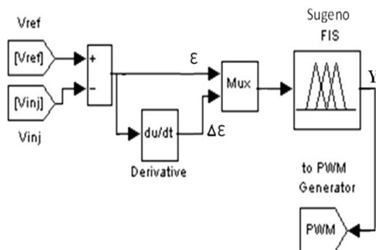
Figure. 4 Fuzzy controller in simulation
