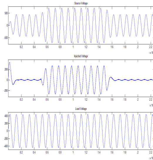
Figure. 5 Voltage waveforms for phase 1
