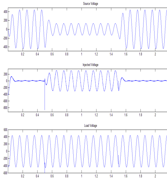
Figure. 6 Voltage waveforms for phase 2
