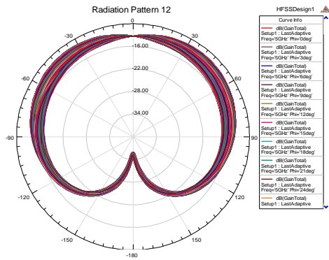
Figure 6.4 Radiation pattern
