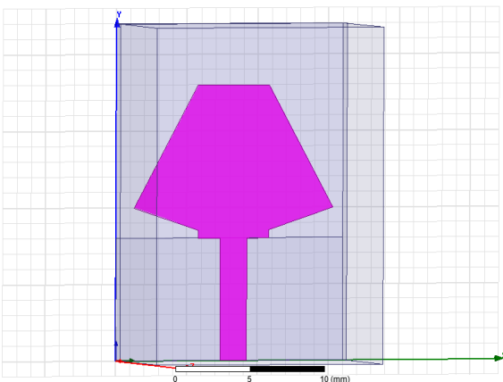
Fig 5.1: DSP UWB antenna without inserting notched region
