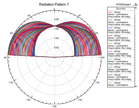
Figure 5.3 Radiation pattern
