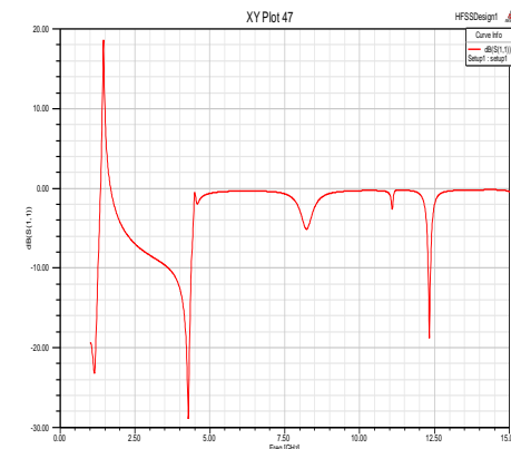
Figure 6.2 Return Loss
