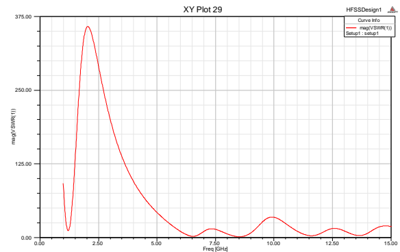
Figure 5.4 VSWR
