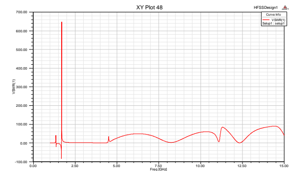
Figure 6.3 VSWR
