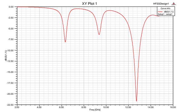
Figure 5.2 Return Loss
