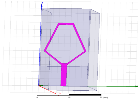
fig 6.1: DSP MINIATURIZED PLANAR MONOPOLE ANTENNA DESIGN;
