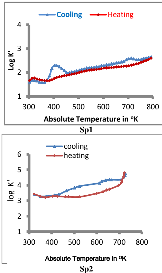
Fig. V: Plots of dielectric constant V/s absolute temperature at 1KHz
