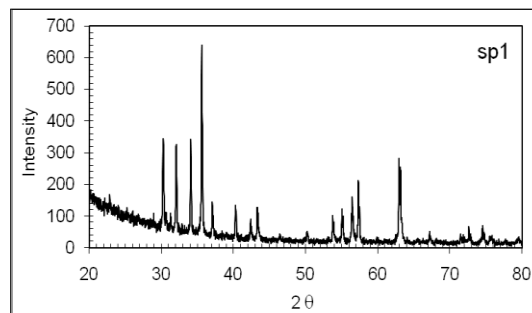
Fig. I(a): X-ray diffraction pattern of SP1
