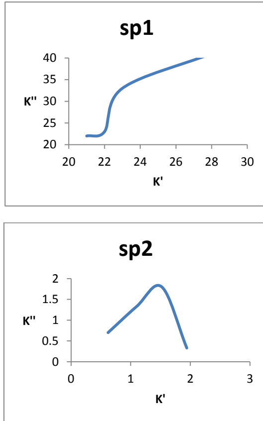
Fig.IV: Cole Cole plots for the spinels
