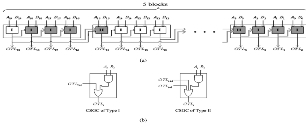
Fig. 3. Control block. (a) Overall architecture and (b) schematic implementations of CSGC.
