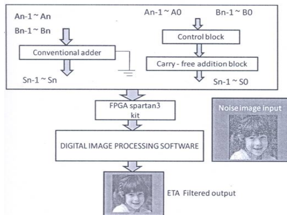
Fig. 4 Block Diagram
