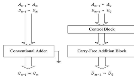
Figure.1: LOW POWER HIGH SPEED ERROR-TOLERANT ADDER
