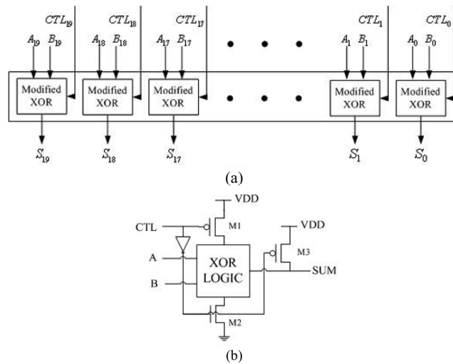
Fig. 2. Carry-free addition block. (a) Overall architecture and (b) schematic diagram of a modified XOR gate.
