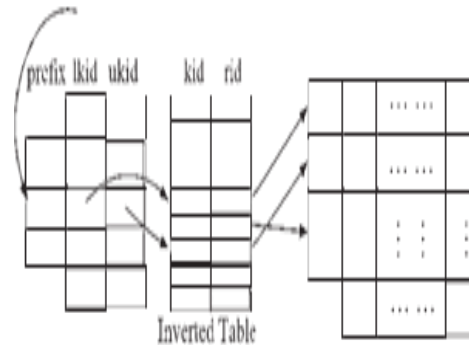
Fig. 1 Using inverted-index table and prefix table to support search-as-you-type.
