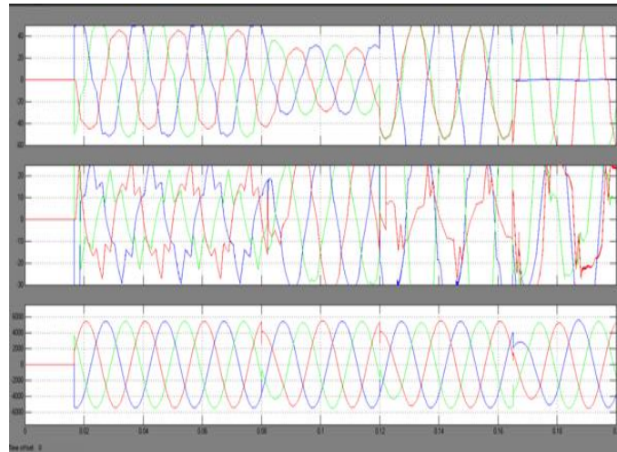
Fig.5 Simulated waveforms for the Scott transformer connection for different Railroad load profiles.
