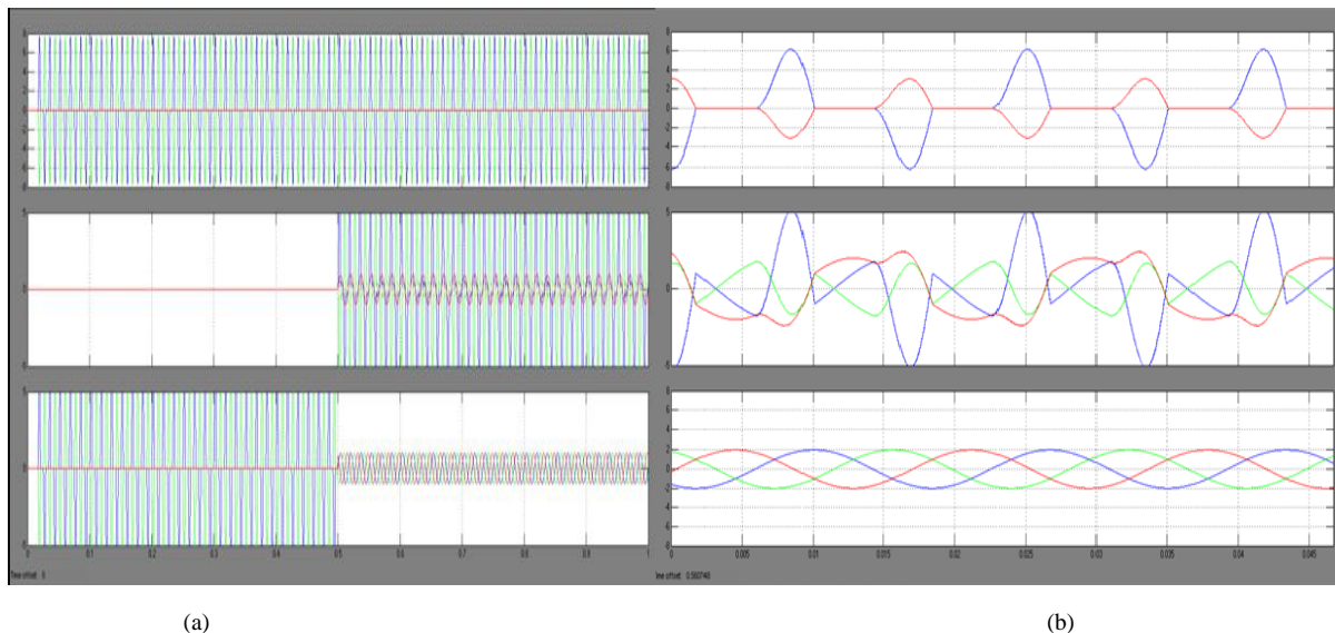
Fig.4. Simulated active filter effect on the power system currents feeding a single phase rectifier load for the Scott and V-V connections (a) V-V (b) Scott.
