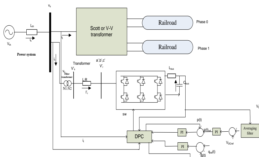
Fig. 1 Proposed Compensation Scheme
