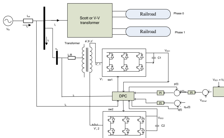
Fig 3.Circuit diagram of proposed multilevel compensation scheme
