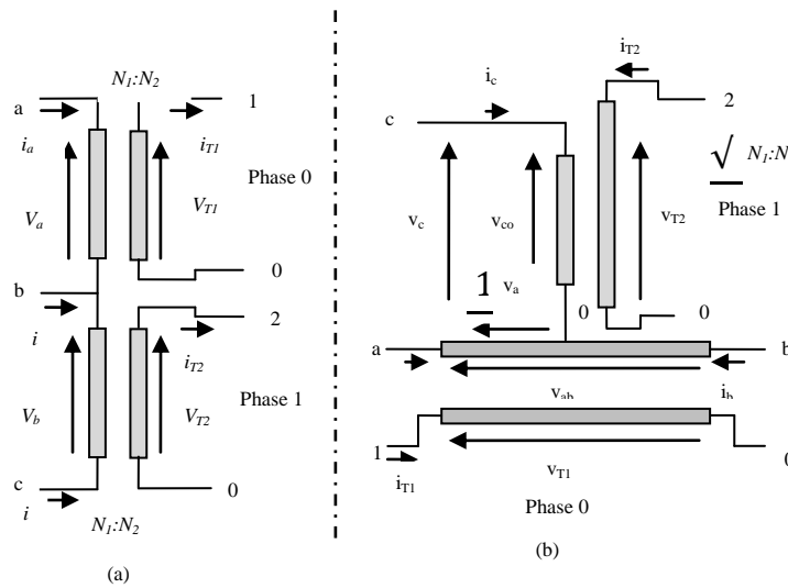
Fig.2 Traction transformer schemes a) V-V transformer b) Scott transformer
