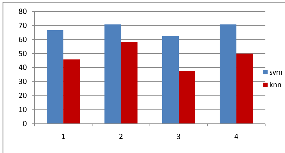
Fig 2. Gabor Orientations Verses Percentage Accuracy
