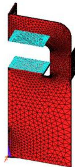
Fig. 10 Load conditions
