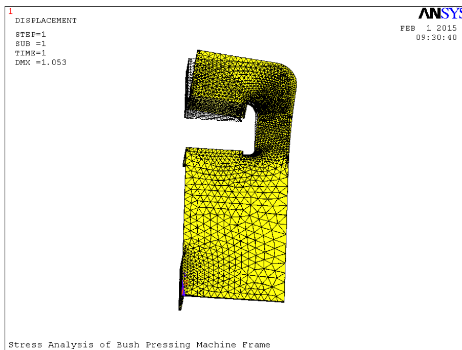
Fig. 11 Deformed shape
