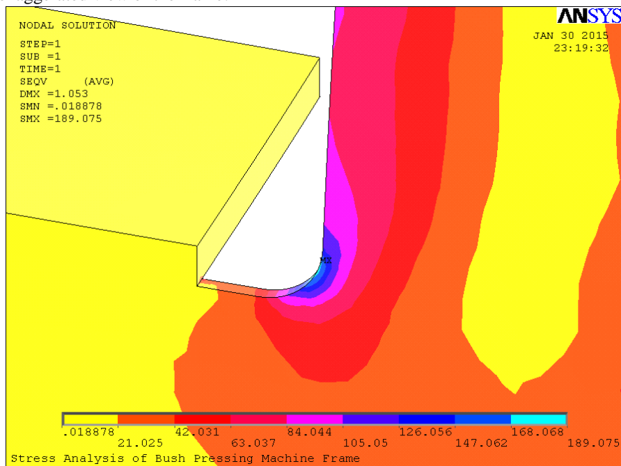
Fig. 13 Exaggerated view showing region of highest stress
