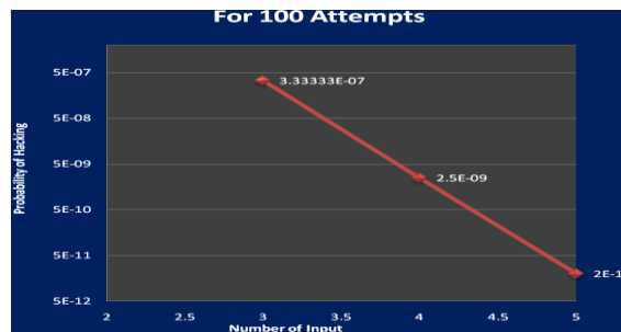
Fig shown the probability of hacking for given number of attempts
