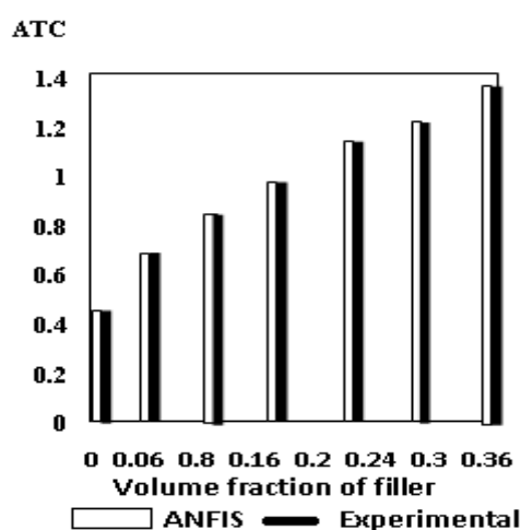
Fig. 8 Effective Thermal Conductivity of boron nitride reinforced high density polyethylene composites
