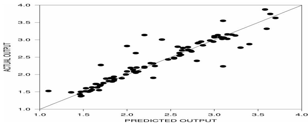
Fig. 6: Actual versus predicted output when final ANFIS model is applied to the 96 testing set.
