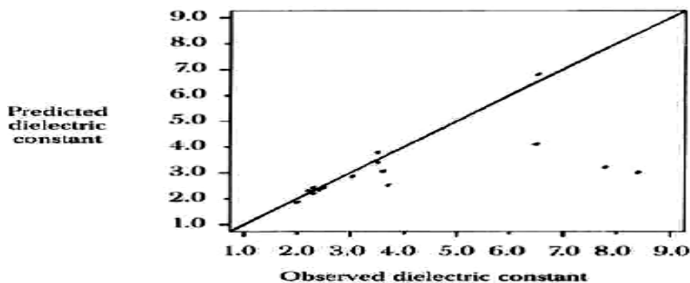
Fig.7 Correlation between the actual values and predicted values by the ANFIS of dielectric constant.
