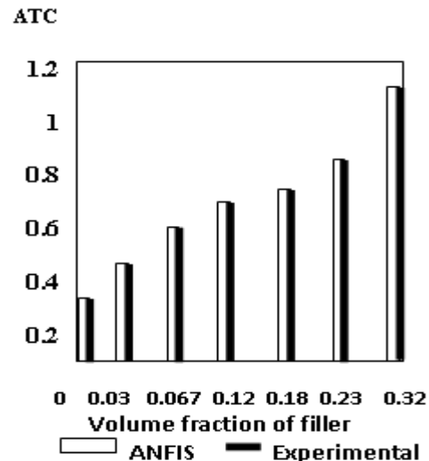
Fig.11 Effective Thermal Conductivity of linear low-density polyethylene with aluminum nitride Composites
