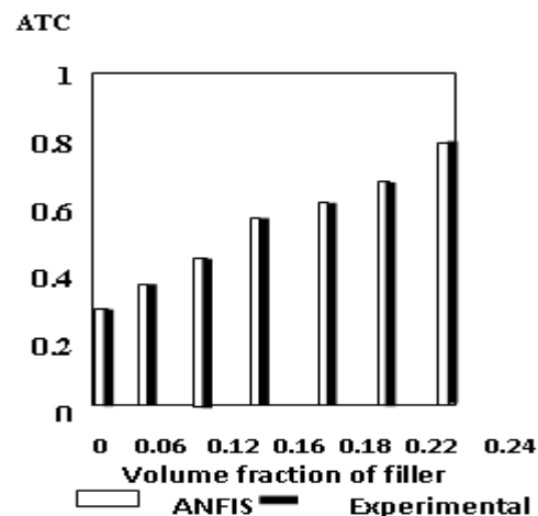
Fig.9 Effective Thermal Conductivity of Copper reinforced low-density polyethylene and linear low-density polyethylene
