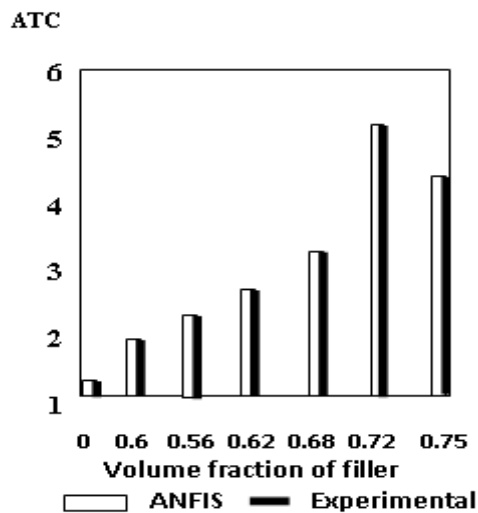
Fig.10 Effective Thermal Conductivity of polyvinylidene fluoride with aluminum nitride Composite.
