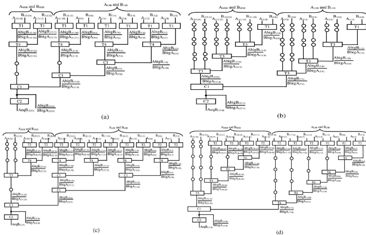
Fig. 4. Examples of novel TB comparators with: (a) and (b) 16-bit operands; (c) and (d) 32-bit inputs.
