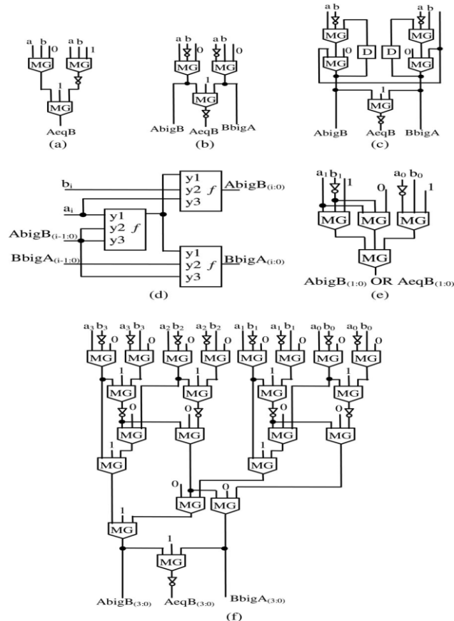
Fig. 1. QCA-based comparators presented in: (a) [22]; (b) [23]; (c) [24];(d) [25]; (e) [26]; (f) [27].
