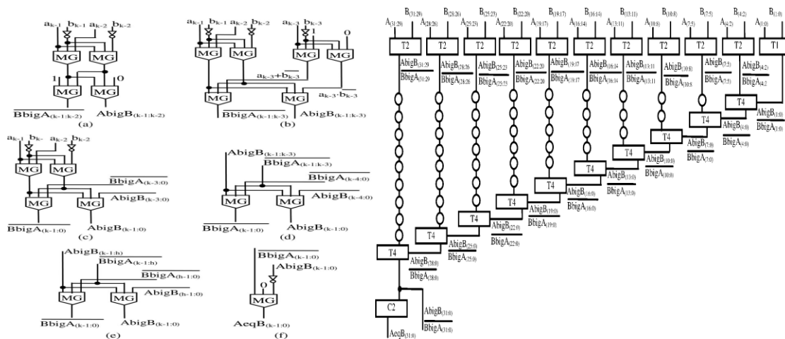
Fig. 2. QCA modules: (a) T1; (b) T2; (c) T3; (d) T4; (e) C1; and (f) C2. Fig. 3. Novel 32-bit CB full comparator.
