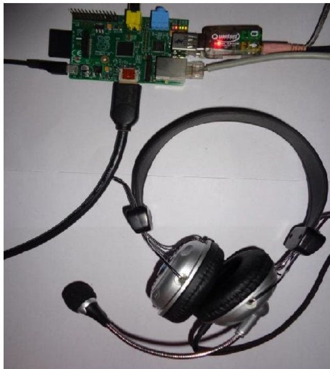
Figure 4.1 Hardware connection of Raspberry-Pi
