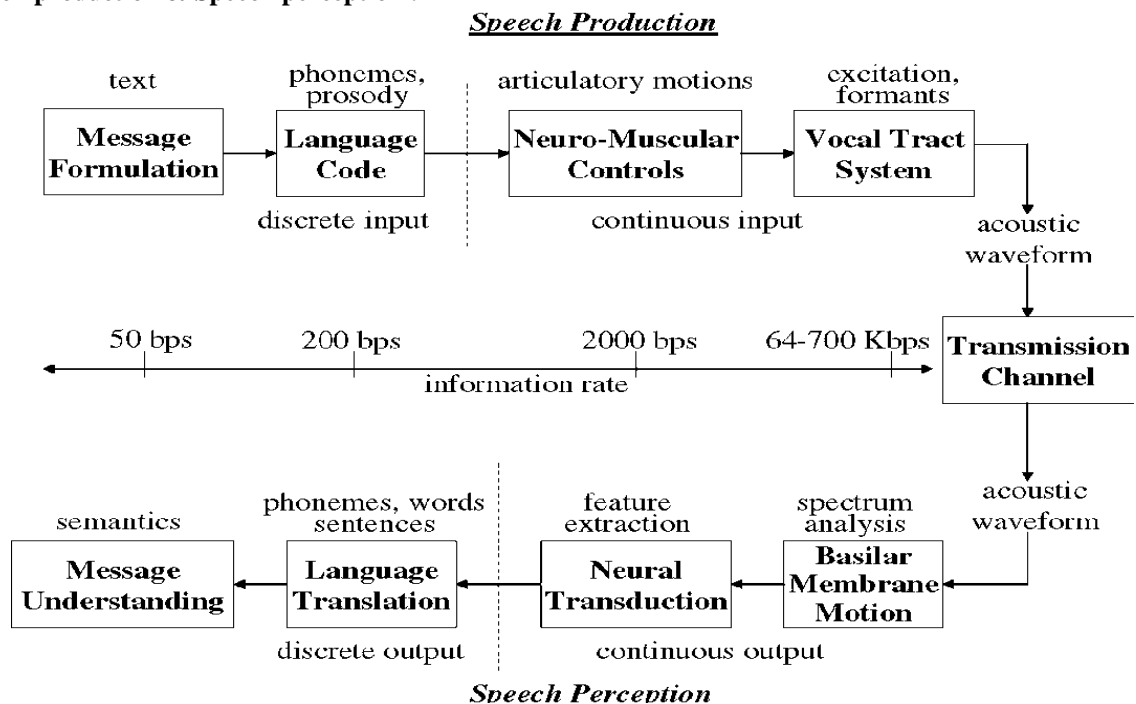
Figure 3.2 Speech Chain
