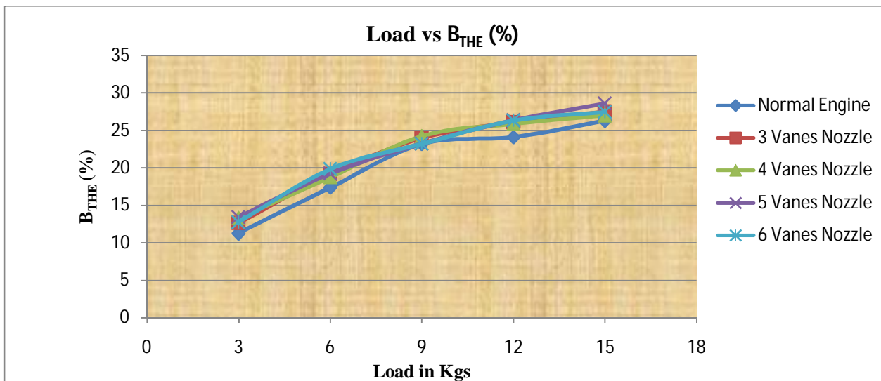
Fig. 4.2: Variation in brake thermal efficiency with change in load
