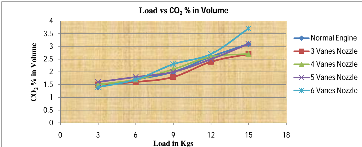
Fig 4.5 : Variation in carbon dioxide with change in load
