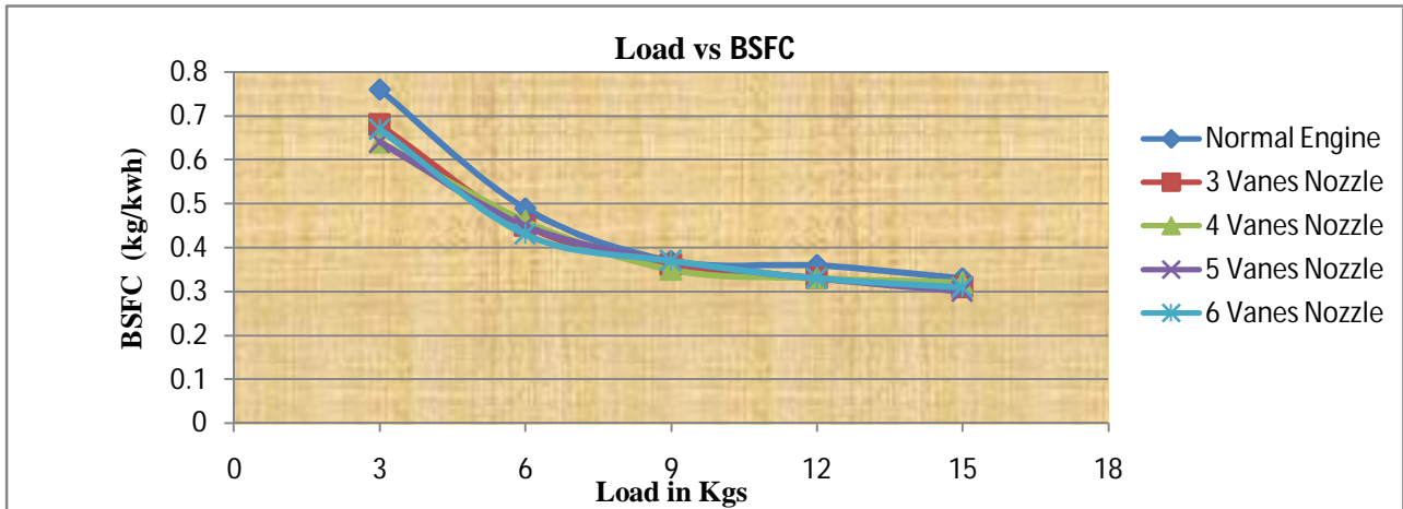
Fig 4.3: Variation in brake specific fuel consumption with change in load
