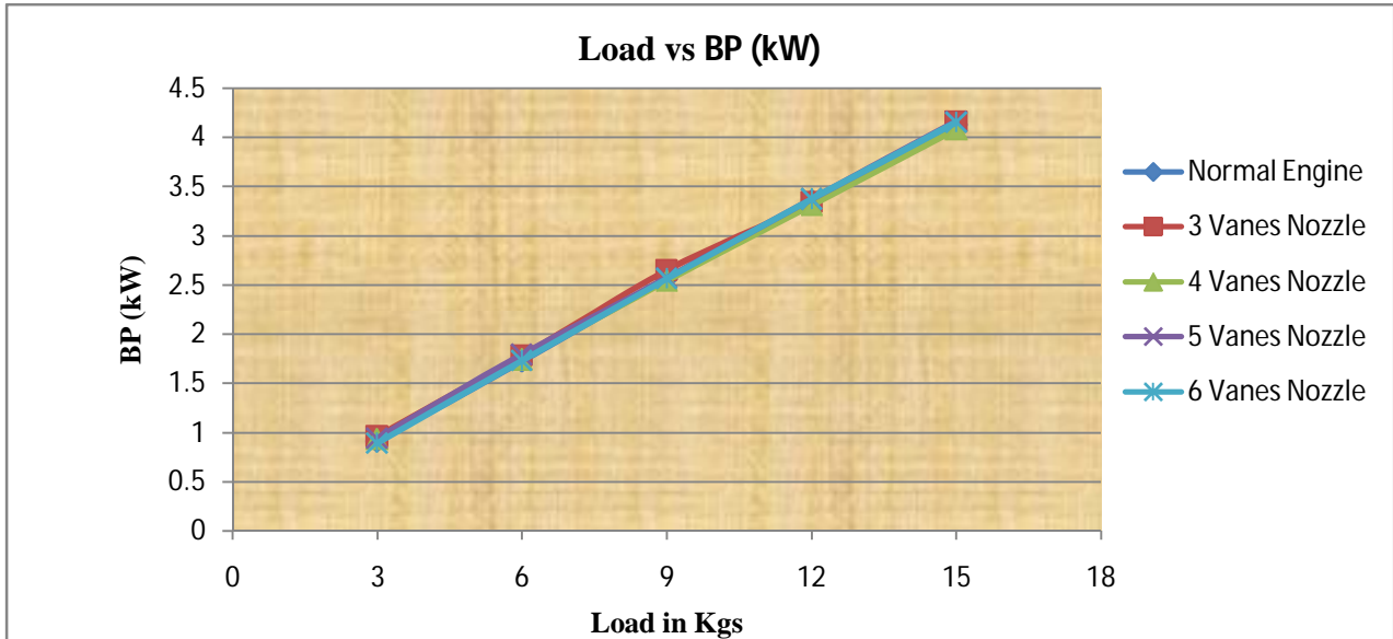
Fig 4.1 Variation in brake power with change in load
