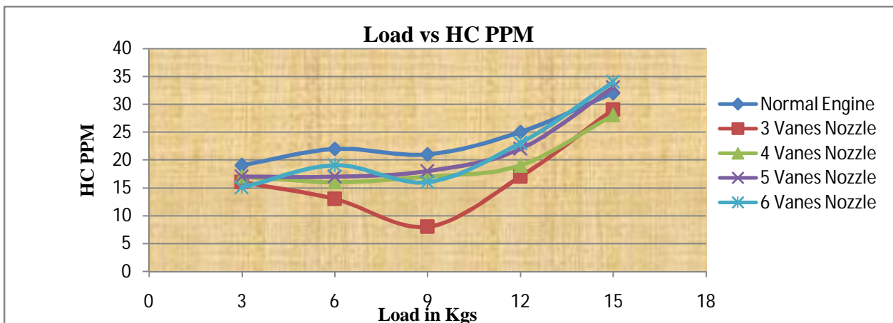
Fig 4.4: Variation in Hydrocarbon with change in load
