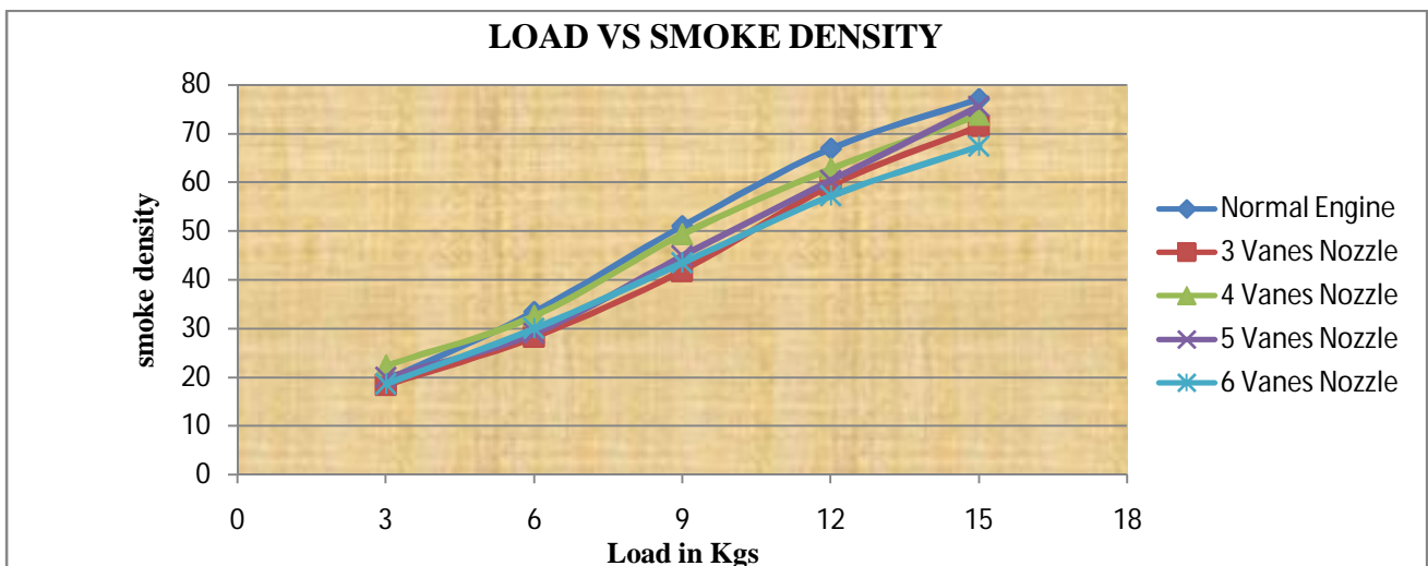
Fig 4.7: Variation in Smoke density with change in load
