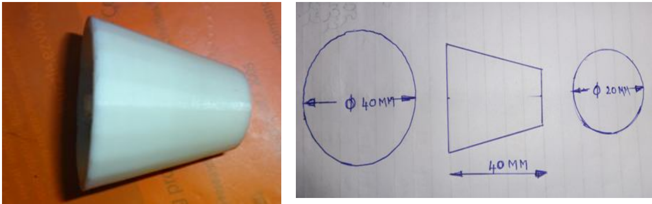
Fig: 3.4 Vane Nozzles and its dimensions
