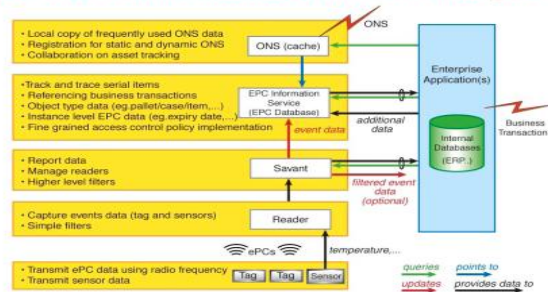
EPC Network Architecture-inside the Enterprise
