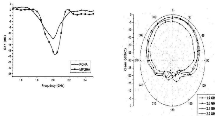
Fig. 3. S11 measurement of the MPQHA compared to the PQHA.
