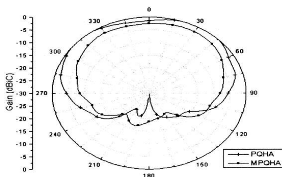
Fig. 6. Elevation angle radiation pattern measurement of MPQHA and PQHA.
