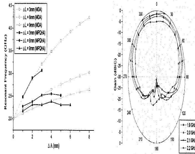
Fig. 2. Comparison of resonant frequency of MDA and MPQHA.
