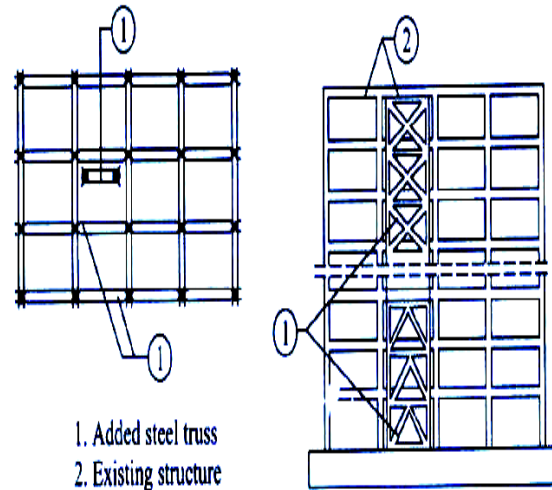
RC Building retrofitted by steel bracing
