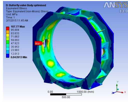
Figure 20: von Mises equivalent stress for valve body optimized disc-opened
