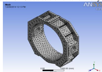
Figure 6: Mesh view for Butterfly valve body optimized design
