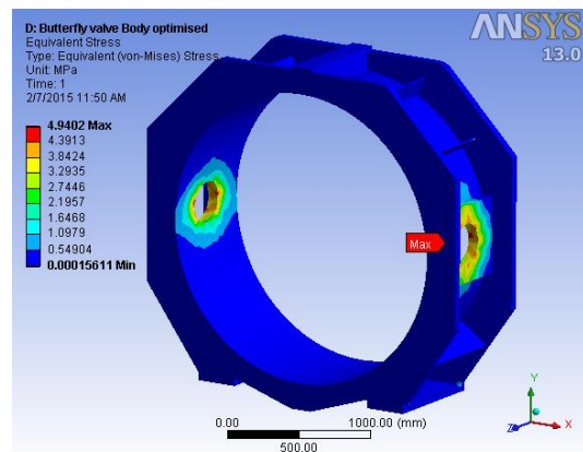
Figure 21: von Mises equivalent stress for valve body optimized disc-close
