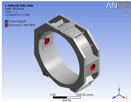
Figure 8: Static structure loading & boundary condition, when valve in fully open condition
