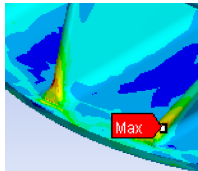
Figure 11: Detail showing the area of maximum von Mises equivalent stress for Butterfly valve disc casted
