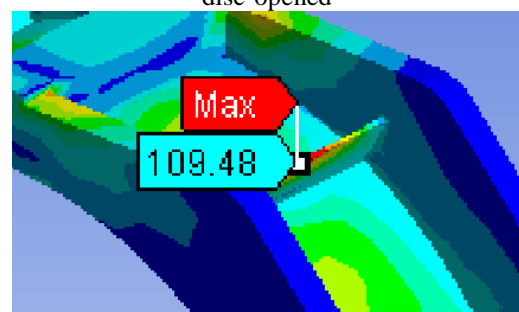
Figure 17: Detail showing the area of maximum von Mises equivalent stress for Butterfly valve body when disc in opened position
