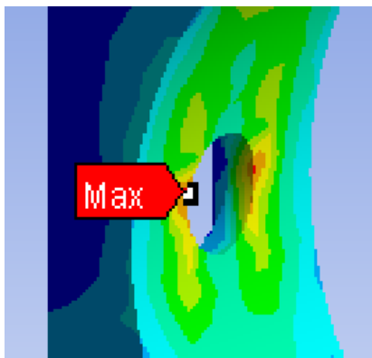
Figure 22: Detail showing the area of maxi von Mises equivalent stress for Butterfly valve body when disc in closed position
