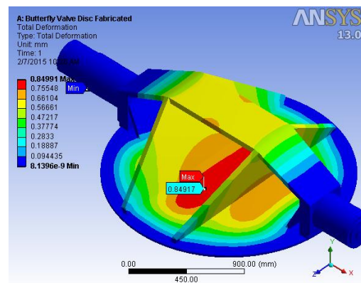
Figure 15: Total deformation for valve disc casted
