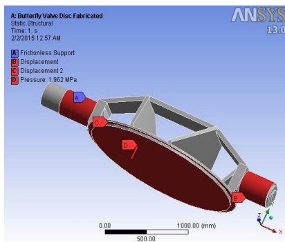
Figure 7: Static structure loading & boundary condition
