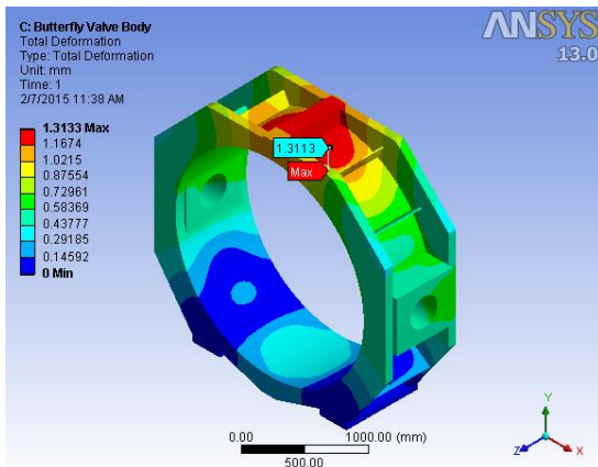
Figure 19: total deformation for valve body disc-closed
