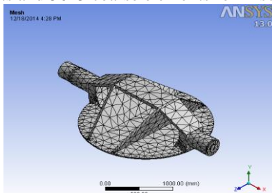
Figure 5: Mesh view for Butterfly valve disc optimized design
