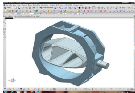
Figure 4: 3D isometric view of Butterfly valve assembly
