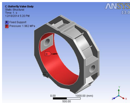
Figure 9: Static structure loading & boundary condition, when valve in fully closed condition
