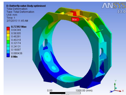
Figure 23: total deformation for valve body disc-closed
