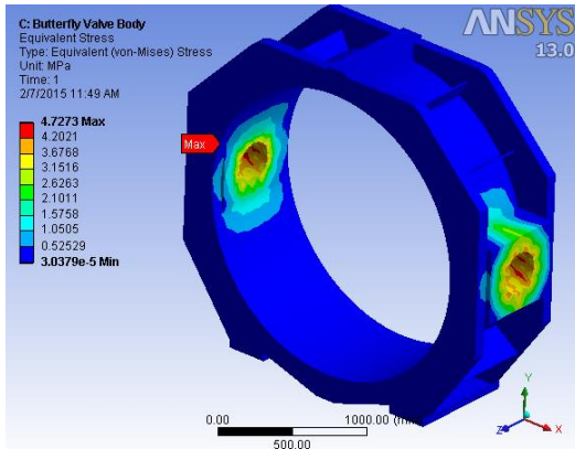
Figure 18: von Mises equivalent stress for valve body disc-closed
