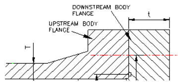
Figure 2: Butterfly valve body section
