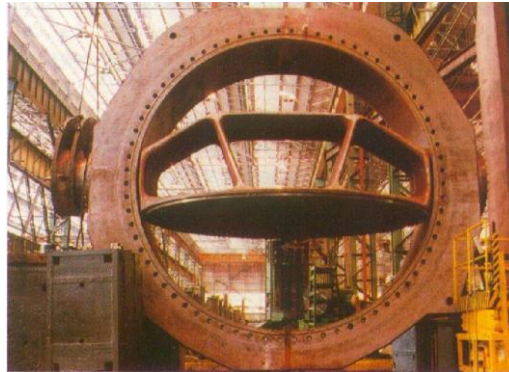
Figure 1: Butterfly valve assembly with biplane disc
