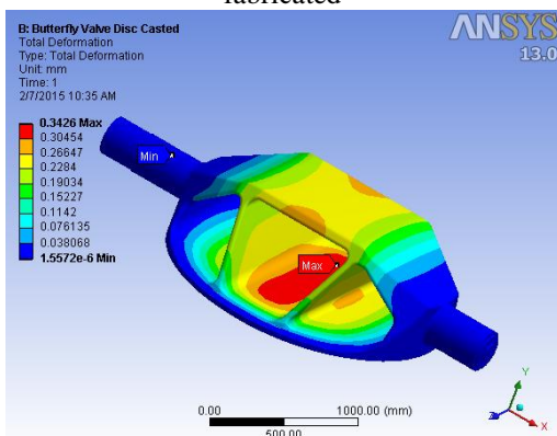
Figure 14: Total deformation for valve disc casted
