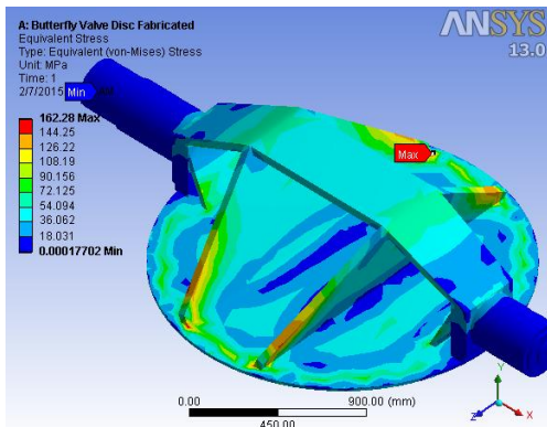
Figure 12: von Mises equivalent stress for valve disc fabricated
