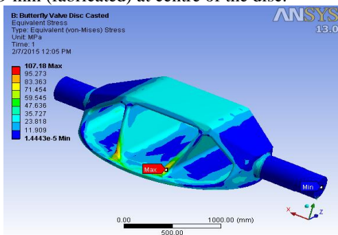
Figure 10: von Mises equivalent stress for valve disc casted
