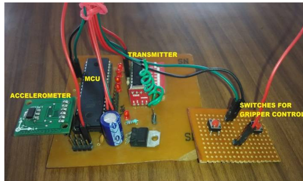
Figure 2: Transmitting End
