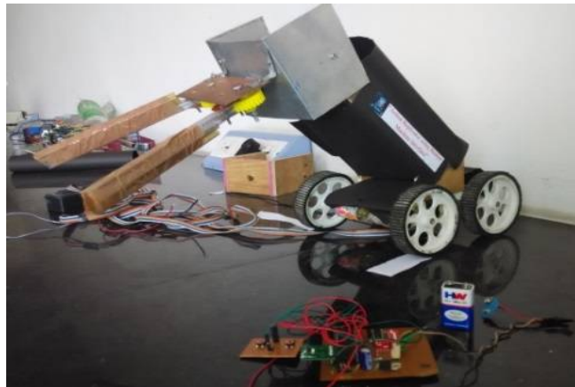
Figure 8: Structure Prototype of Robotic Arm
