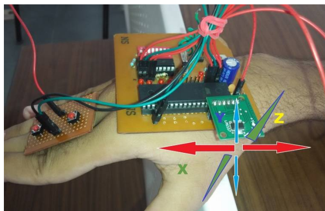
Figure 3: Accelerometer returns X, Y, Z acceleration in sensor's frame of reference
