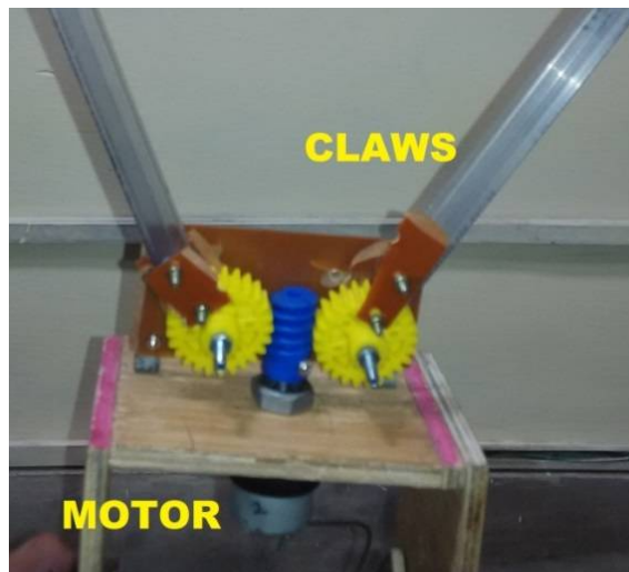
Figure 4: Gripper Mechanism
