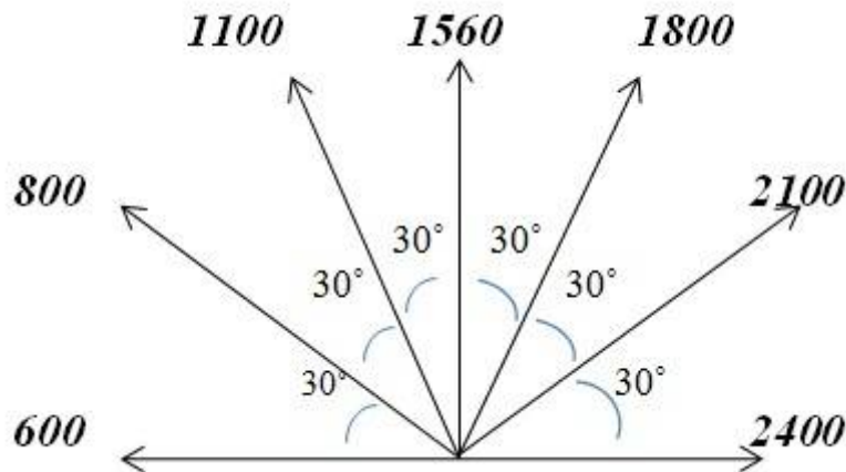
Figure 6: Angle Separation Corresponding to PWM Values.
