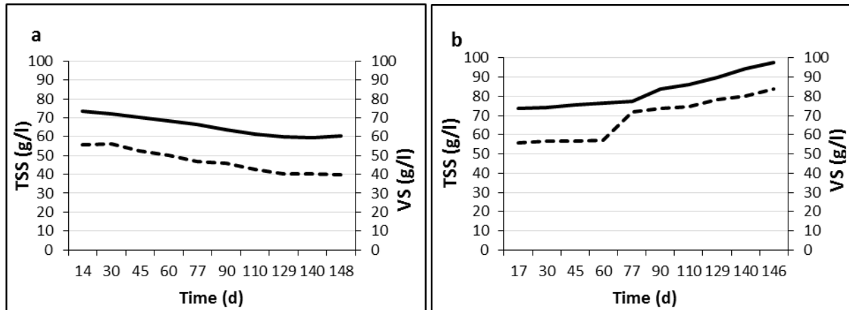
Fig.5. Total Suspended Solids (TSS) and Volatile Solids (VS) in the sludge during the digestion of slaughterhouse wastewater at high micro-aerobic (a) and aerobic conditions (b). (——) TSS, (-----) VS
