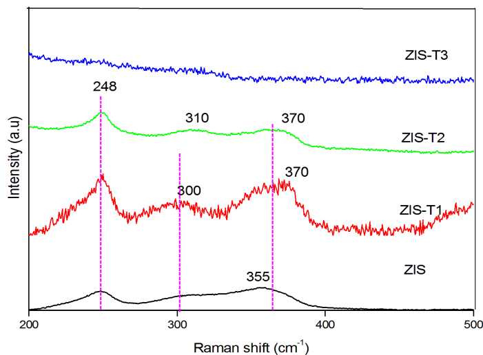
Fig. 2 Raman study of the as-deposited and annealed ZIS film
