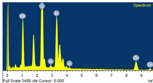
Fig.7 EDAX Spectrum of the as-deposited ZnIn 2 S 4 (ZIS) thin film
