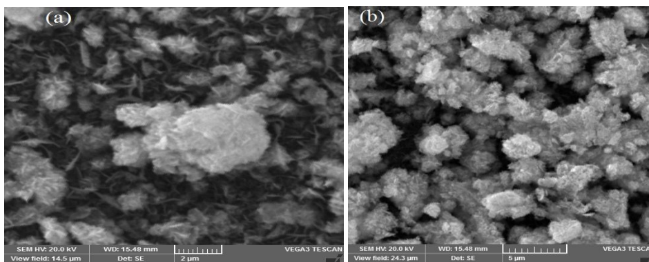
Fig.8 FESEM as-deposited ZnIn 2 S 4 (ZIS) thin film with different magnification such as (a) 2 μm, (b) 5 μm.
