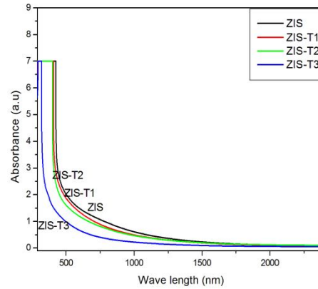
Fig.4 Absorption of the as-deposited and annealed ZIS film
