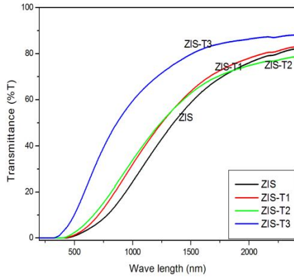
Fig.3 Transmittance of the the as-deposited and annealed ZIS film
