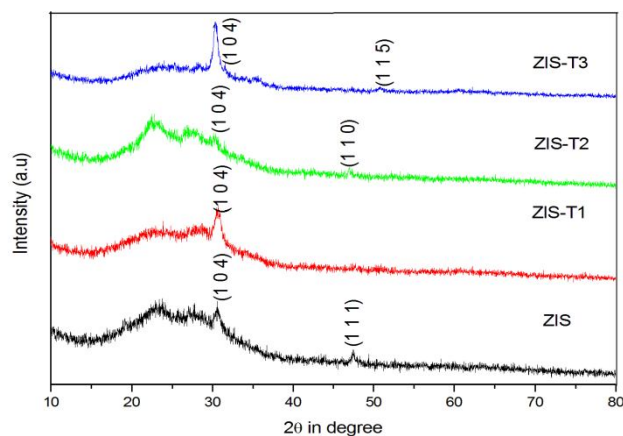
Fig. 1. Structural characterization of the as-deposited and annealed ZIS film
