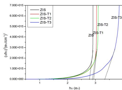
Fig.6 Direct band gap of the as-deposited and annealed ZIS film
