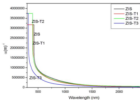
Fig.5 Absorption coefficient of the as-deposited and annealed ZIS film
