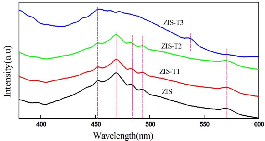
Fig.9 PL Spectrum of the of the as-deposited and annealed ZIS film
