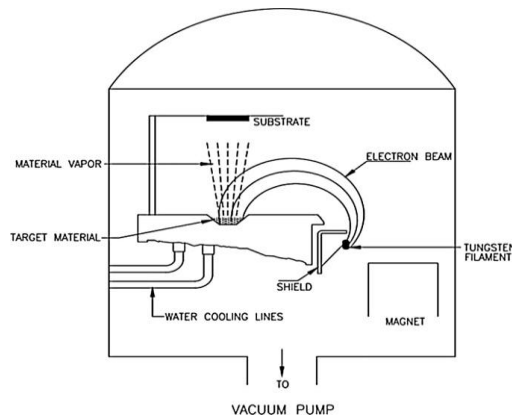
FIGURE 2.11. PVD PROCESS
