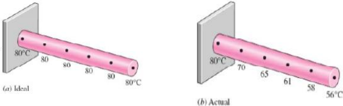
FIGURE 2.4 FIN EFFICIENCY
