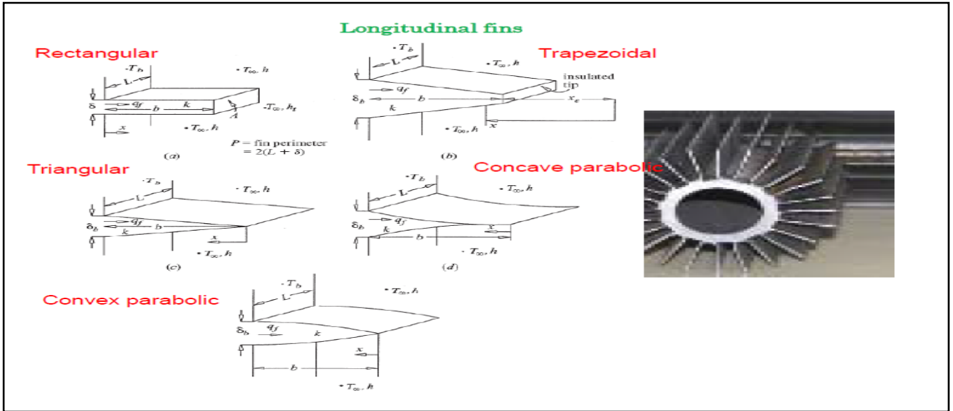
FIG 2.1 GEOMETRIES OF FINS
