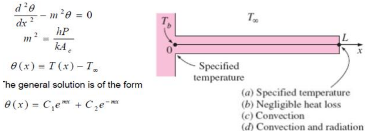
FIG 2.3 BOUNDARY CONDITIONS
