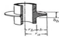
Hyperbolic profile
