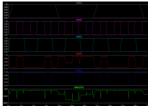
Fig.3.Modified SRAM Operation under Stress
