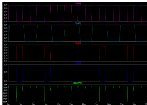
Fig.1. CMOS Normal Operation
