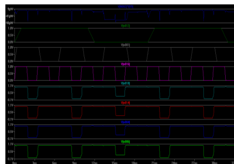
Fig.4.Modified SRAM Operation under Stress with Array
