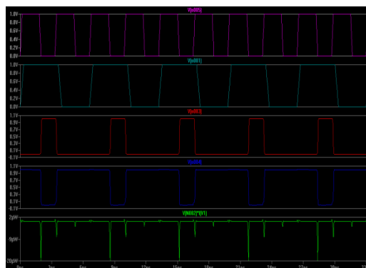
Fig. 2 .CMOS under Stress Mode
