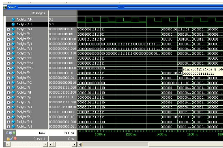
Fig 5.1 Output waveform for Transposed Polyphase decimation filter using BFD multiplier
