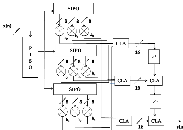
Fig 3.1. Transposed Decimation Filter structure
