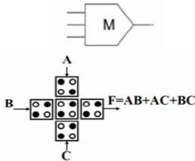
Figure.5 Majority Gate
