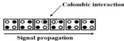
Figure.2 Signal Flow
