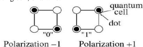
Figure.1 QCA Cell
