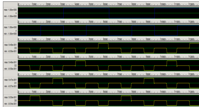
Fig.10 Simulation Output
