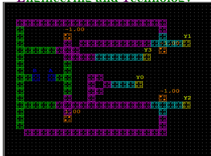
Figure.7 Multilayer design
