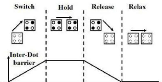
Figure.4 Clock Phase
