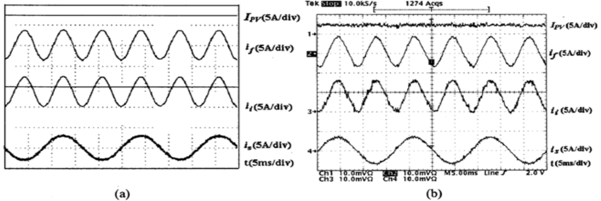
Fig 3(a) Simulated result input and output current of the proposed conversion system. Fig 3(b) Experimental result of input and output current of the proposed conversion system.
