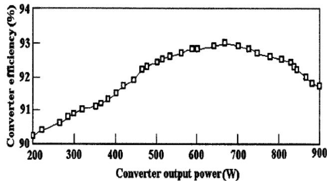
Fig. 10. Efficiency of the proposed conversion system.
