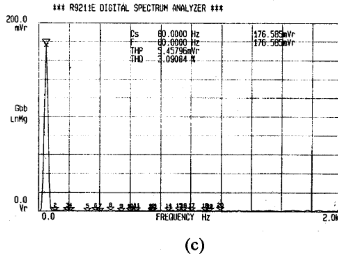
Fig. 7 Solar generator mode. (a) Waveforms of i_s, i_o, and i_t . (b) Waveforms of v_s, and i_s . (c) Current spectrum of i_s .
