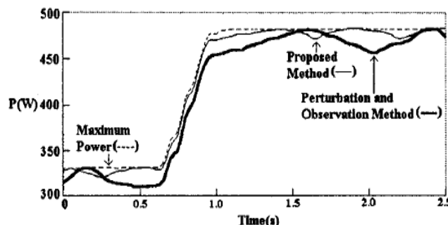
Fig. 6. Solar array output power of the proposed method and the perturbation and observation method
