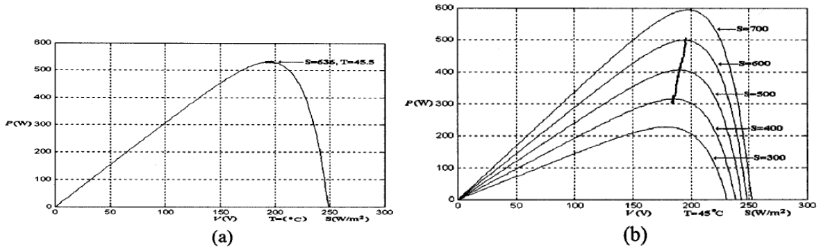
Fig. 5. MPPT measurement of the proposed method. (a) Constant insolation. (b) Varying insolation.
