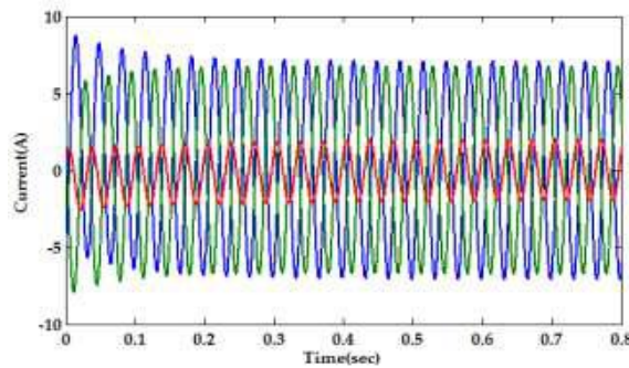
Figure k: Current during LLG fault
