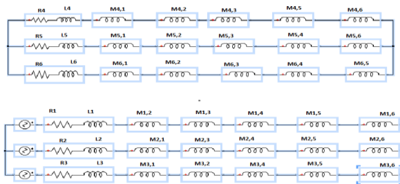
Figure a: Magnetic Shield
