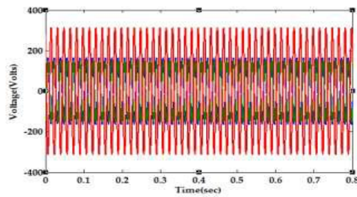
Figure h: Fault Voltage during LL fault
