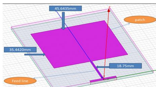
Figure 1. Rectangular Patch Antenna Geometry
