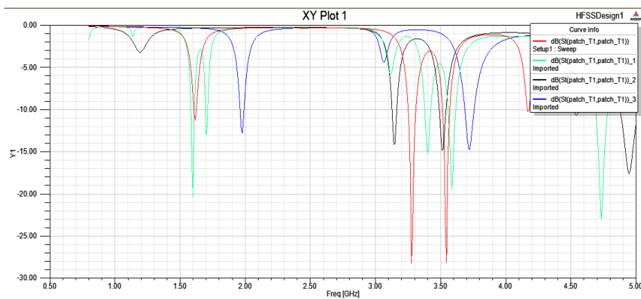
Figure 3. Simulated Return Loss Plot of rectangular patch and three iteration models.
