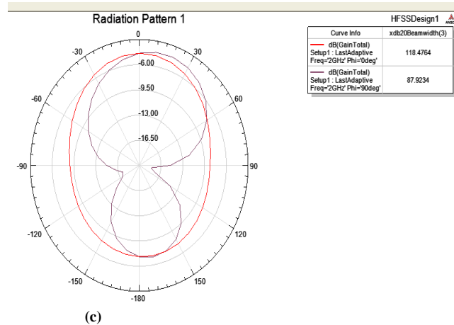
Figure 5. (a) Second Iteration Model (b) Return Loss Plot and (c) Radiation Pattern of Second Iteration Model
