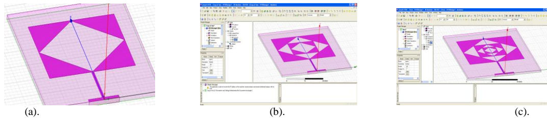
Figure 2. (a) First Iteration Model (b) Second Iteration Model (c) Third Iteration Model
