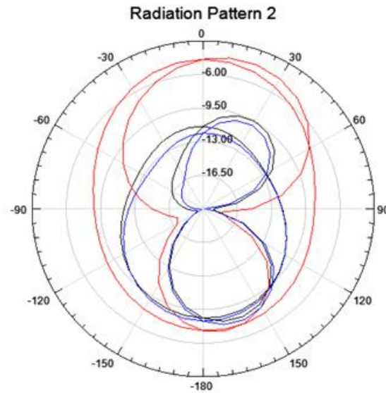
Figure 4. Radiation Pattern of all three Iteration Models
