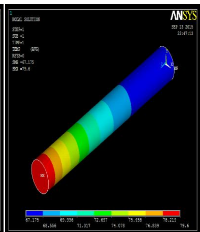
Fig:5.2(c) Result of heat transfer of copper pin fin
