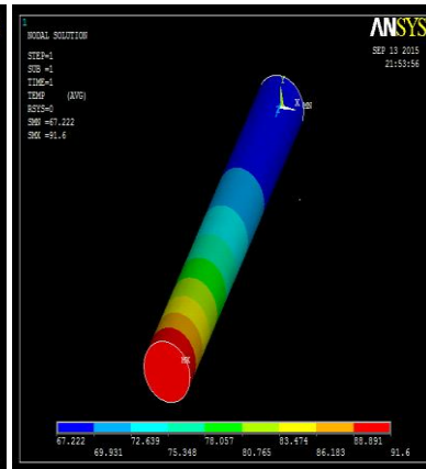
Fig:5.1(c) Result of heat transfer of Aluminium pin fin
