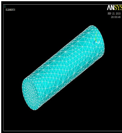
Fig 5.3(b) Meshed view of brass+ aluminium
