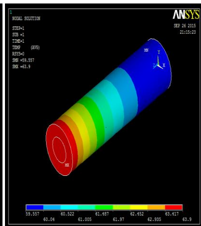
Fig:5.4(c) Result of heat transfer pin fin of copper + aluminium pin fin
