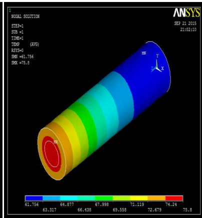
Fig:5.3(c) Result of heat transfer of brass+ aluminium pin fin
