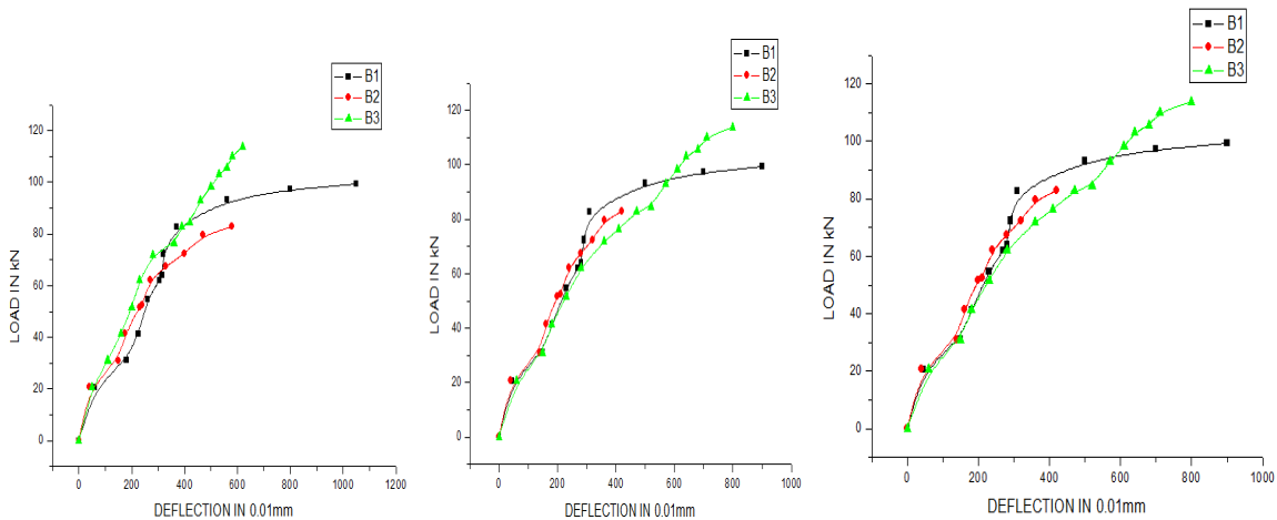
FIG 7:LOAD V/S DEFLECTION OF BEAMS AT RESPECTIVE PORTIONS
