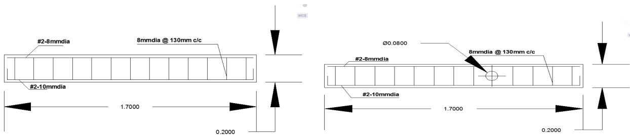
FIG 1: NORMAL SOLID RC BEAM FIG 2: RC BEAM PROVIDING TRANSVERSE CIRCULAR OPENING
