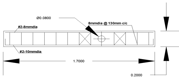
FIG 3: RC BEAM PROVIDING TRANSVERSE CIRCULAR
