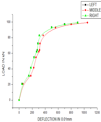
FIG 4:LOAD V/S DEFLECTION RELATION OF B1 BEAM
