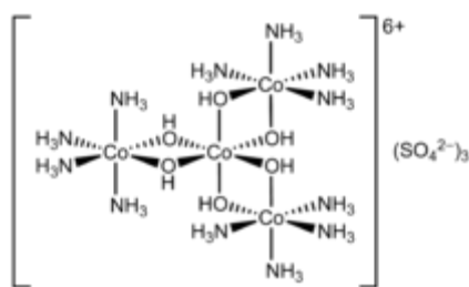
Structure of Hexol
