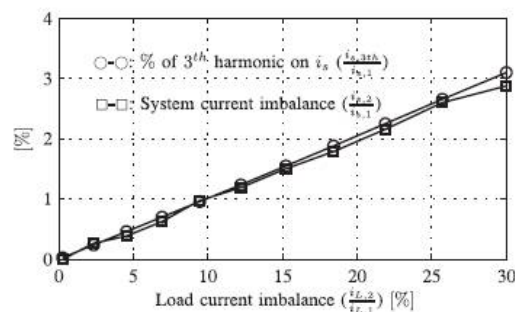
Fig. 6. Relationship between permissible unbalance load currents, the corresponding third-order harmonic content, and system current imbalance (with respect to positive sequence of the system current, i_{s,1} ).
