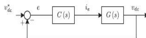
Fig. 7. DC-voltage control block diagram.
