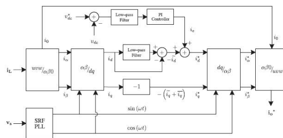
Fig. 5. dq -based current reference generator block diagram.
