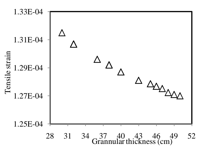
Figure 7. Strain variations with granular layer ( h_2 ) thickness.
