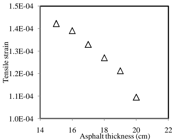
Figure 6. Strain variations with asphalt layer ( h_1 ) thickness.
