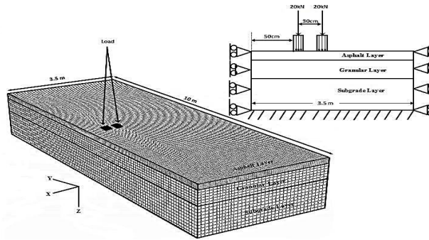
Figure 1. 3-layered asphalt pavement structure.
