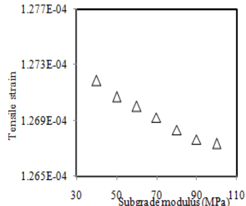
Figure 5. Strain variations with modulus ( E_3 ) of subgrade layer.
