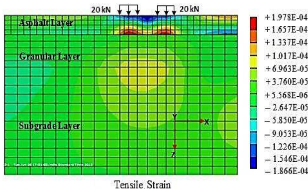
Figure 2. Contour plots of tensile strain in 3-layered pavement structure.
