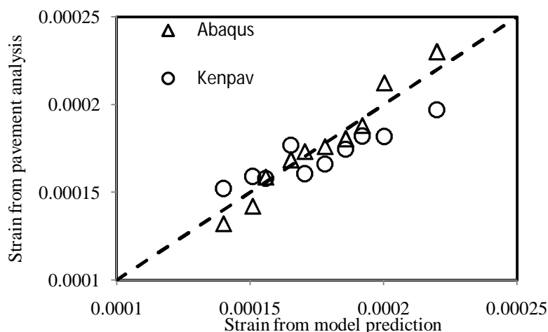
Figure 8. Comparison of tensile strain parameter in asphalt pavements.
