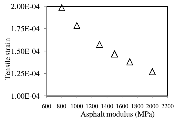
Figure 3. Strain variations with modulus ( E_1 ) of asphalt layer.
