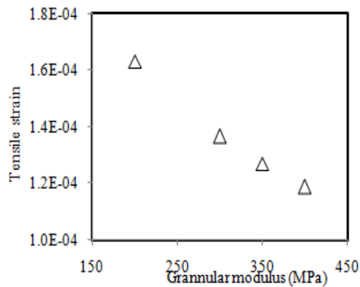
Figure 4. Strain variations with modulus ( E_2 ) of granular layer.
