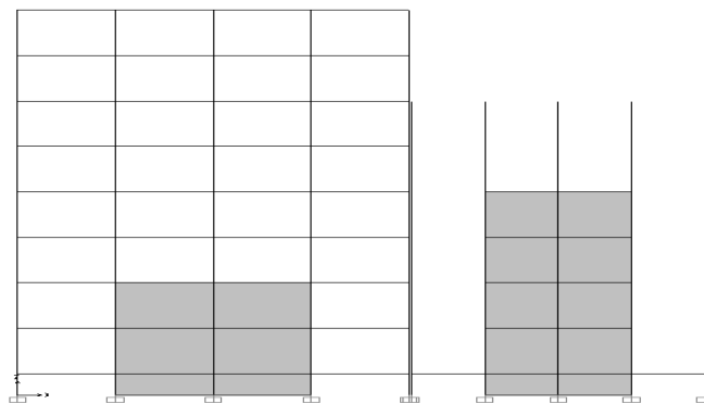
Figure 6: Elevation view of structures having RC Wall of reduced length at mid two panels in X Direction
