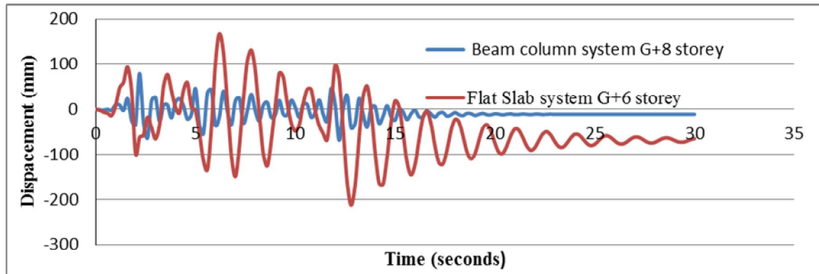
Figure- 3: Time vs. displacement graph of beam column system adjacent to flat slab system at sixth-floor roof level without any RC wall.
