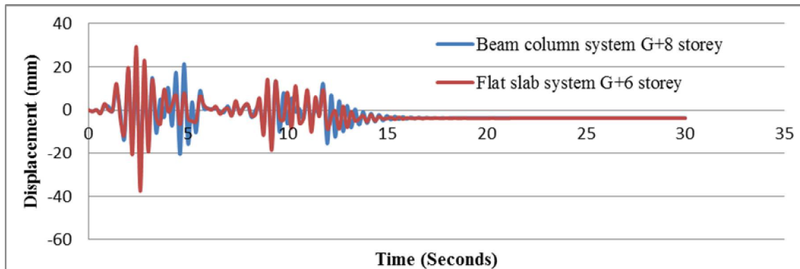
Figure 5: Time vs. displacement graph of beam column system adjacent to flat slab system at sixth-floor roof level with RC wall
