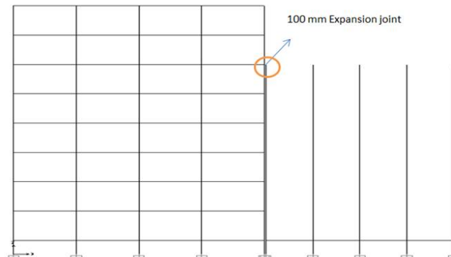
Figure-2: Elevation view of beam column system adjacent to flat slab system without any RC wall
