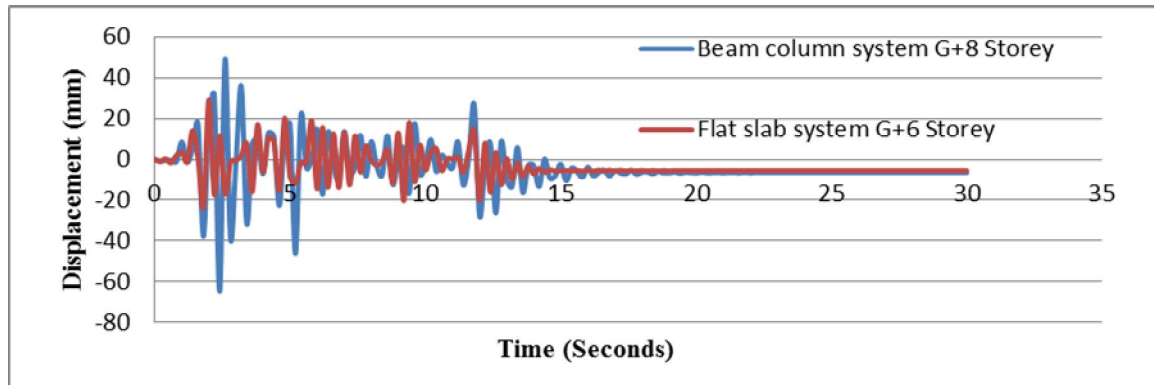
Figure 7: Time vs. displacement graph for both the buildings after reducing the length of the RC wall
